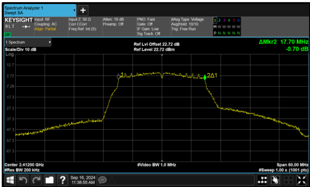
Figure 147 - 802.11n HT20 Maximum 99% OBW
