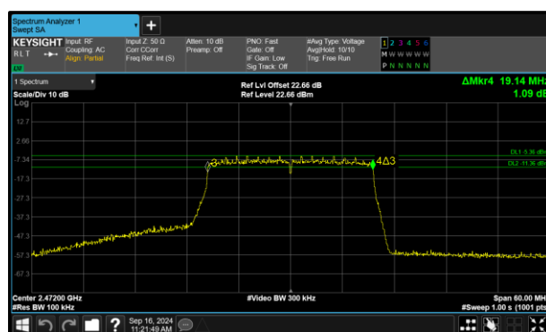
Figure 133 - 802.11ax HE20 SU Maximum 6 dB EBW
