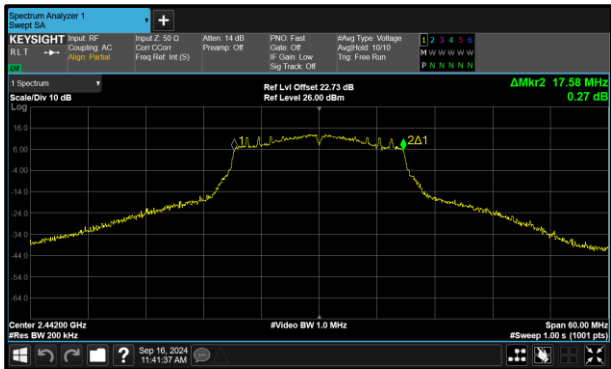
Figure 146 - 802.11n HT20 Minimum 99% OBW
