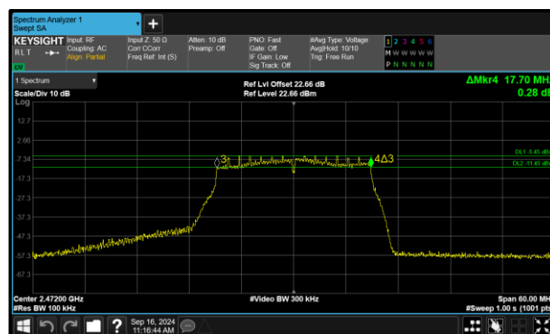
Figure 131 - 802.11n HT20 Maximum 6 dB EBW
