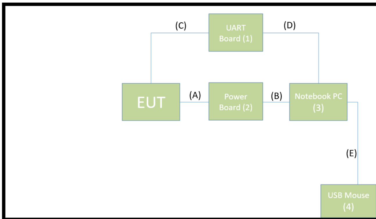
Connection Diagram
