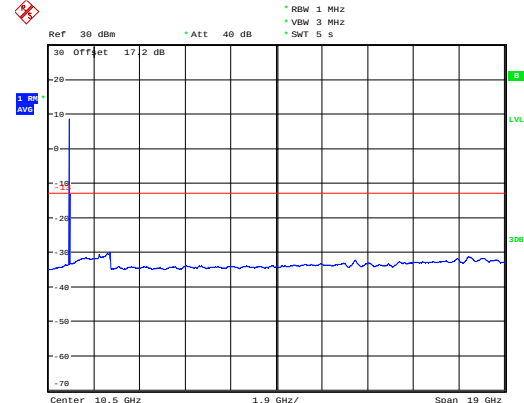
NB-IOT Band 2 CH-Middle 1GHz ~20GHz
