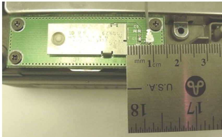
Distance between Left-Side WLAN Antenna & GPRS Dipole Antenna
