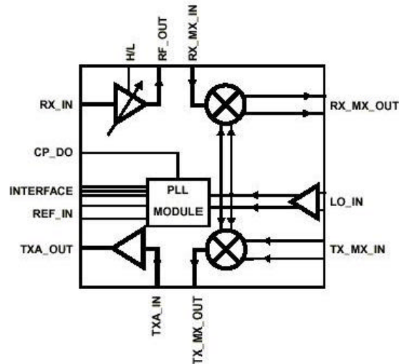
Simplified Block Diagram for HFA3683A
