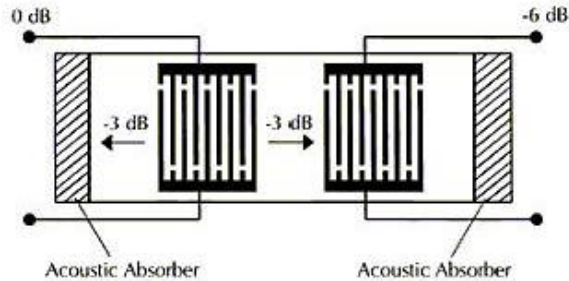
Figure 2. Simple transversal SAW filter configuration
