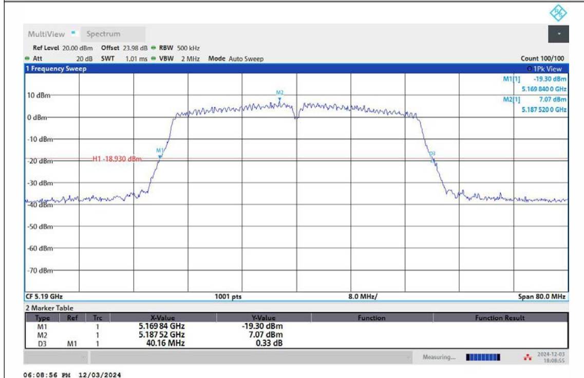
11AC40MIMO-Ant2-5190
