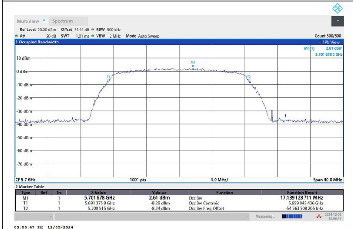
11A-Ant2-5700
