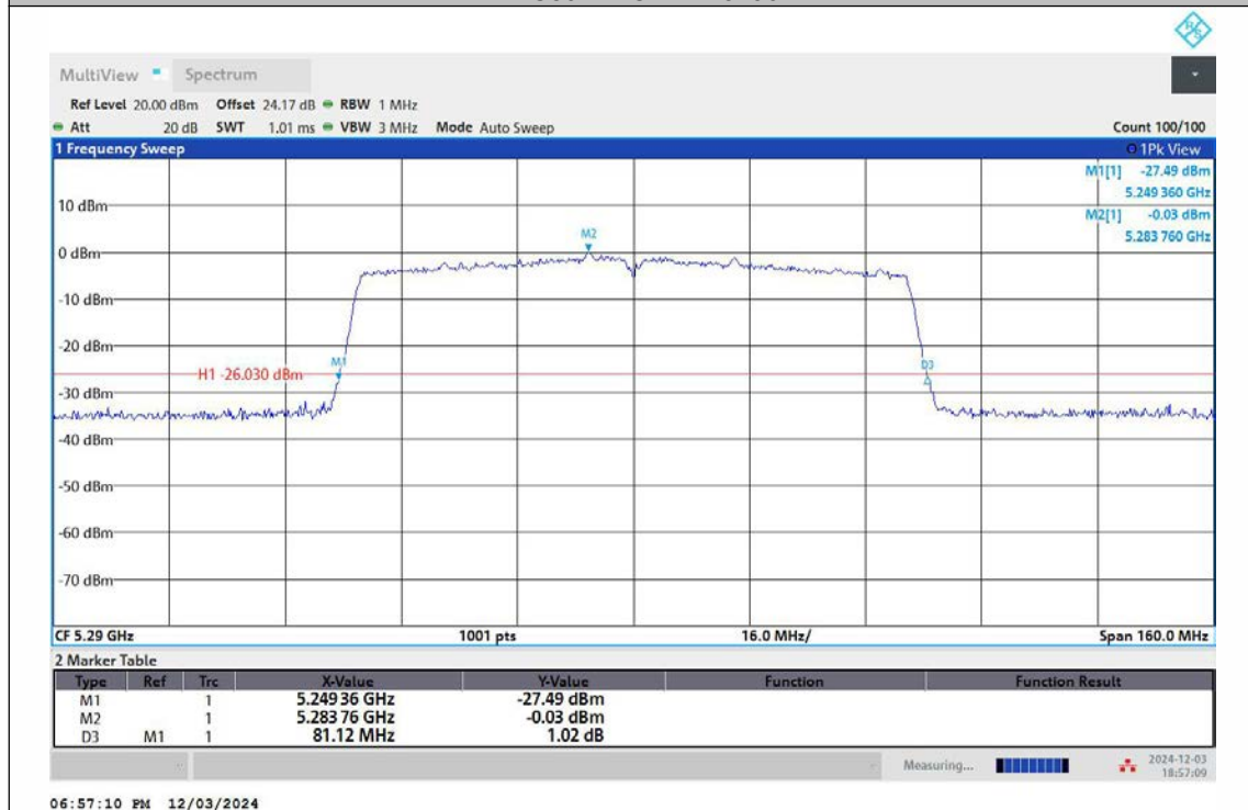
11AC80MIMO-Ant2-5290
