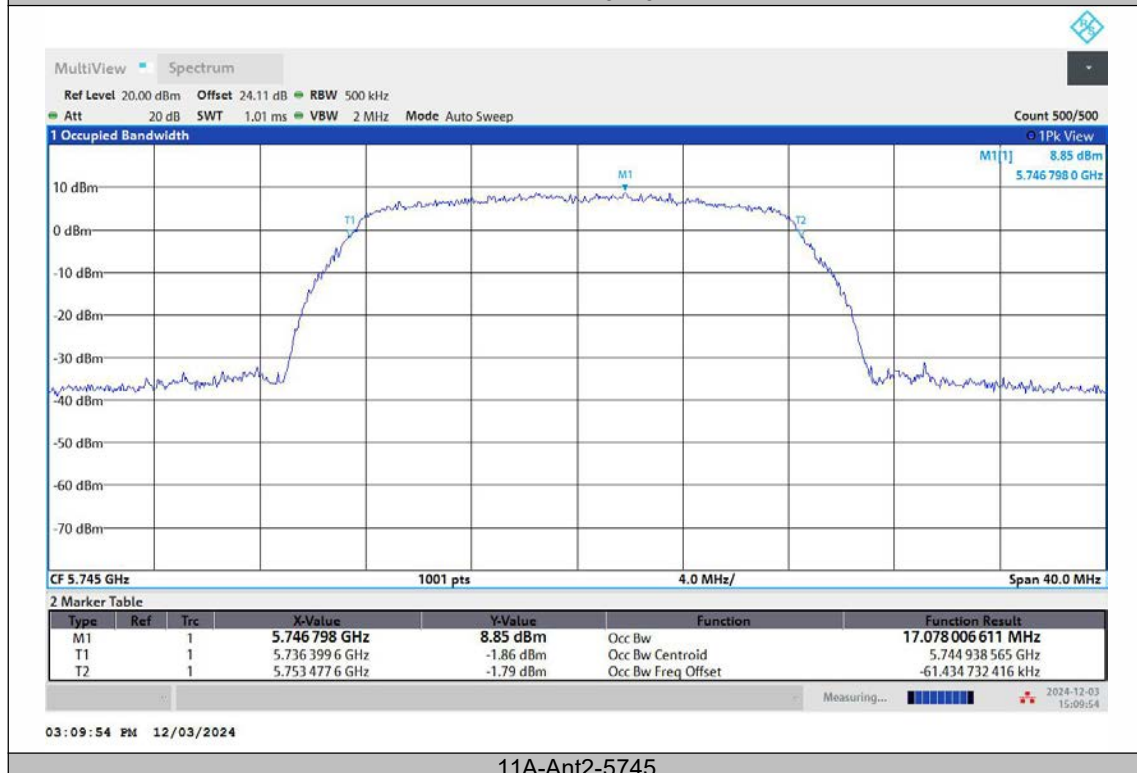
11A-Ant2-5745
