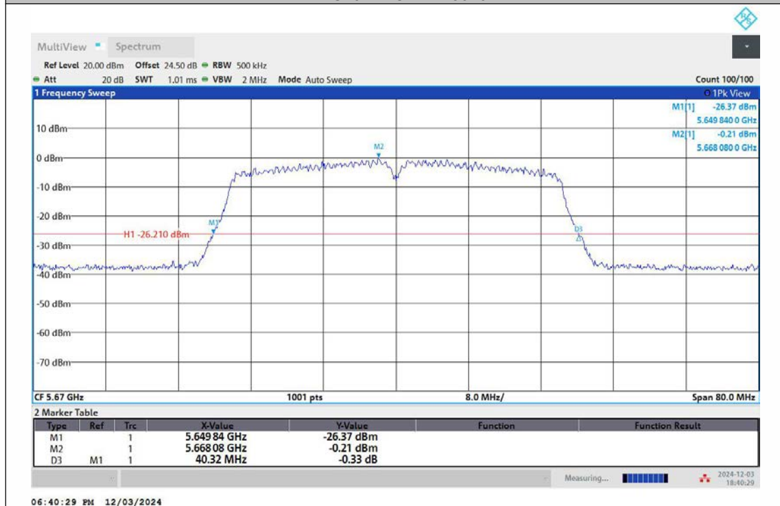
11AC40MIMO-Ant2-5670
