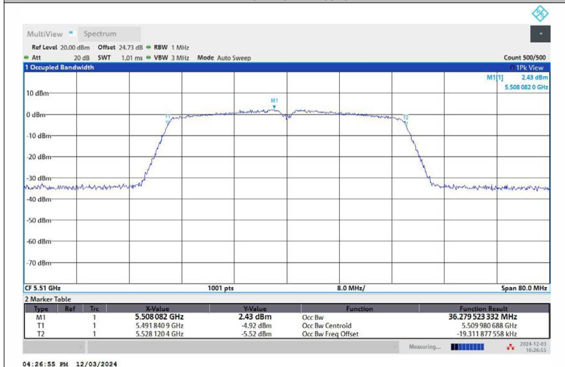
11N40MIMO-Ant2-5510
