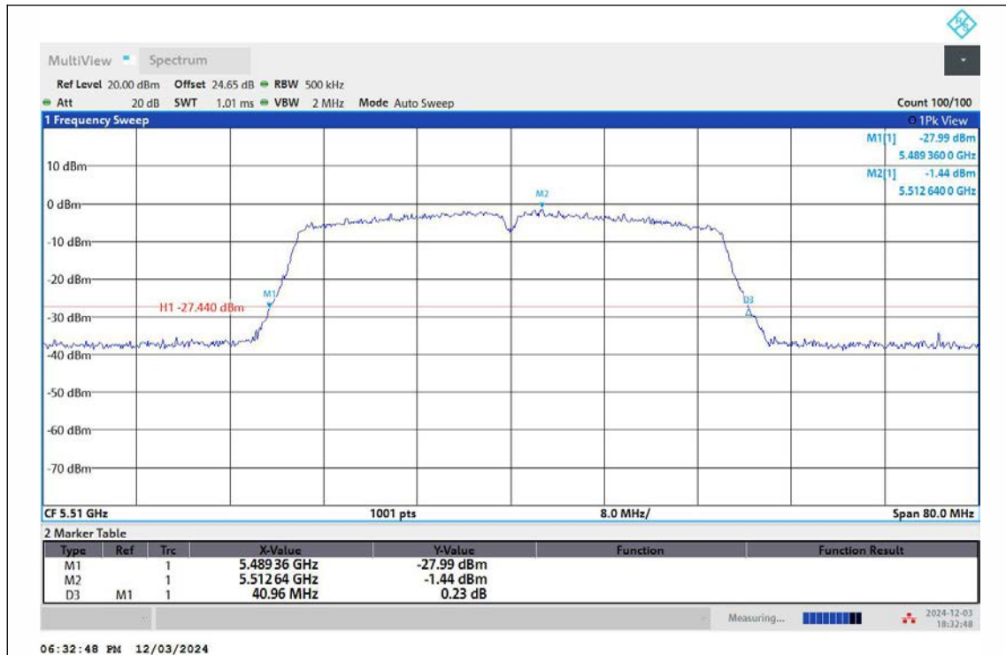
11AC40MIMO-Ant1-5510
