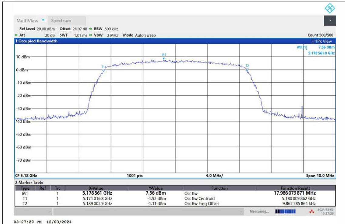
11N20MIMO-Ant1-5180
