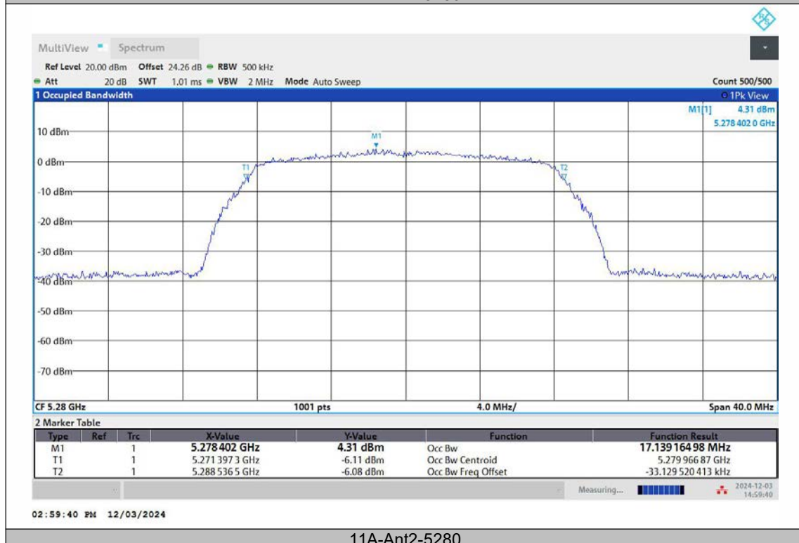
11A-Ant2-5280
