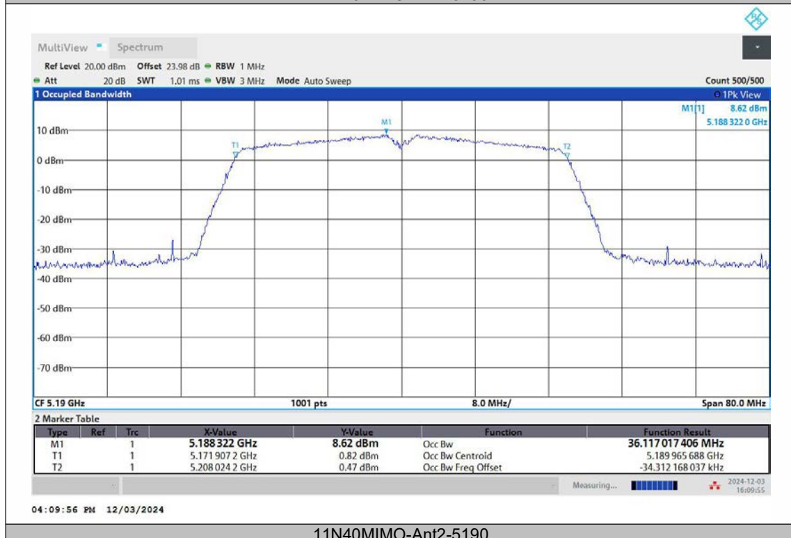
11N40MIMO-Ant2-5190
