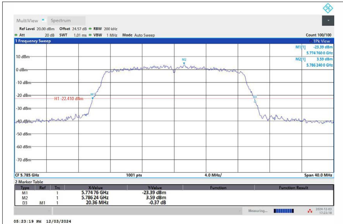
11AC20MIMO-Ant1-5785
