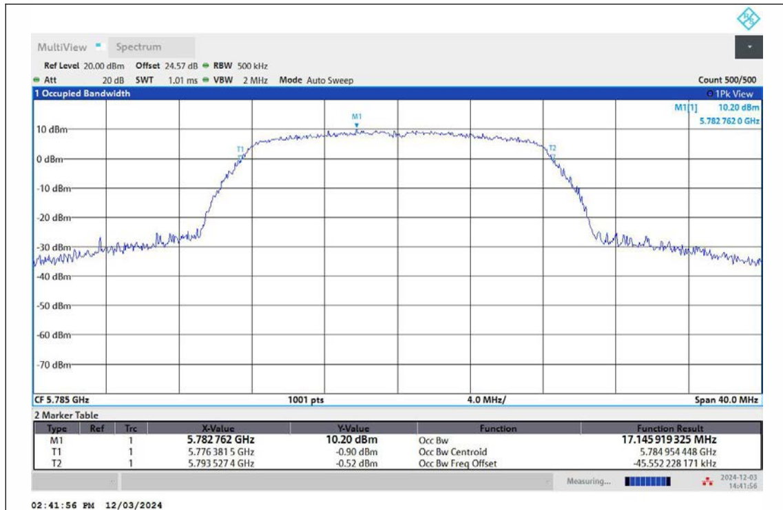
11A-Ant1-5785
