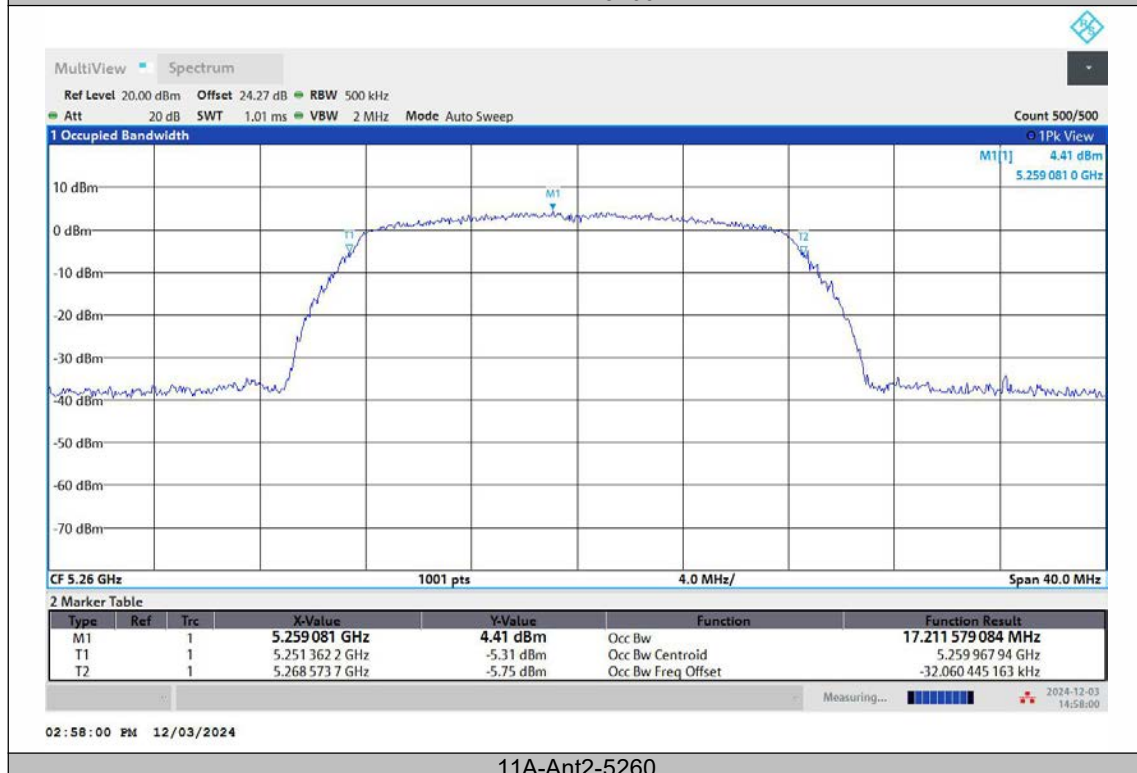
11A-Ant2-5260
