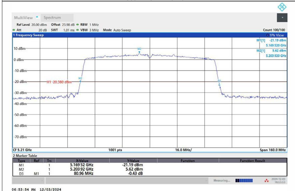
11AC80MIMO-Ant2-5210
