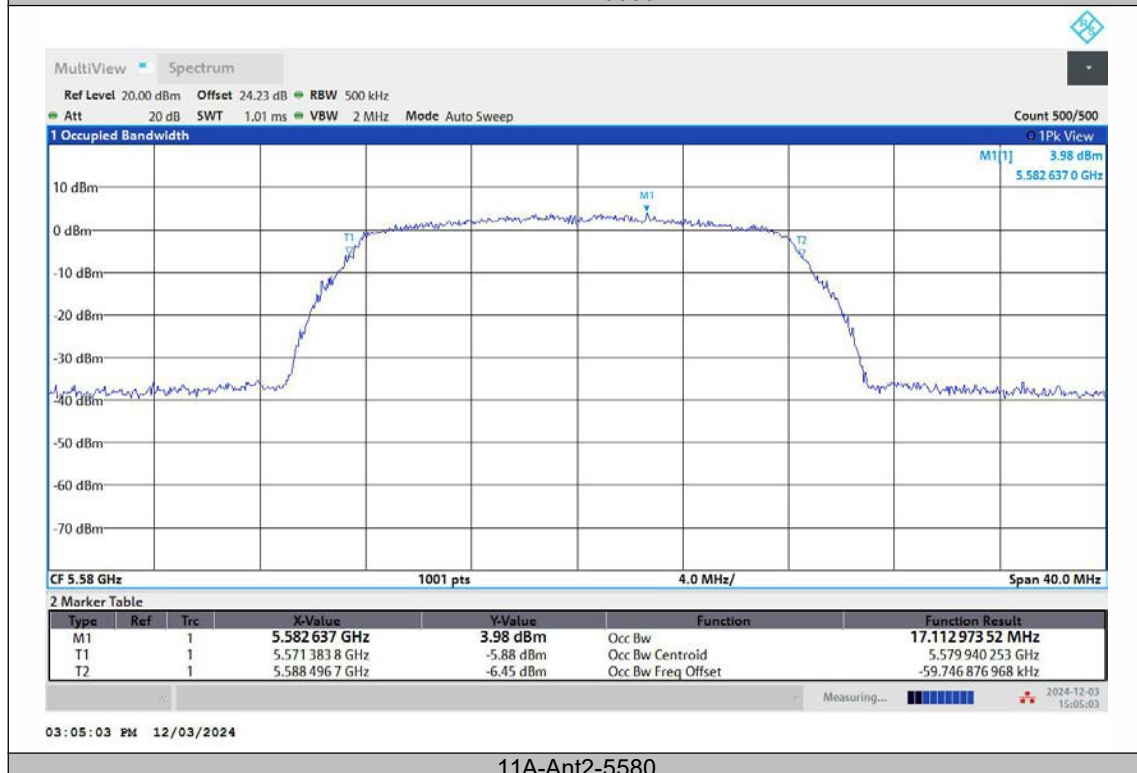
11A-Ant2-5580
