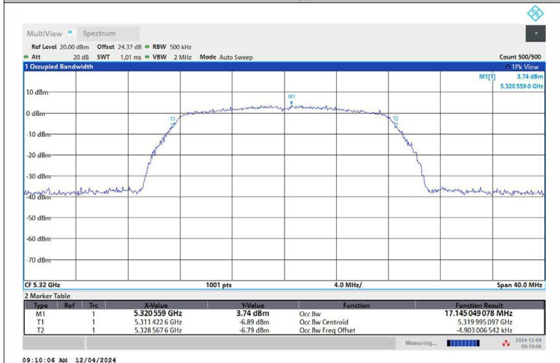
11A-Ant2-5320
