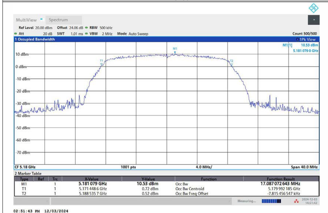
11A-Ant2-5180
