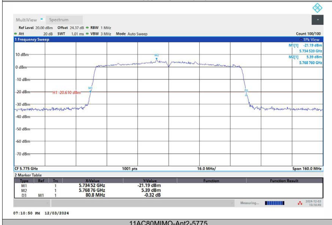
11AC80MIMO-Ant2-5775
