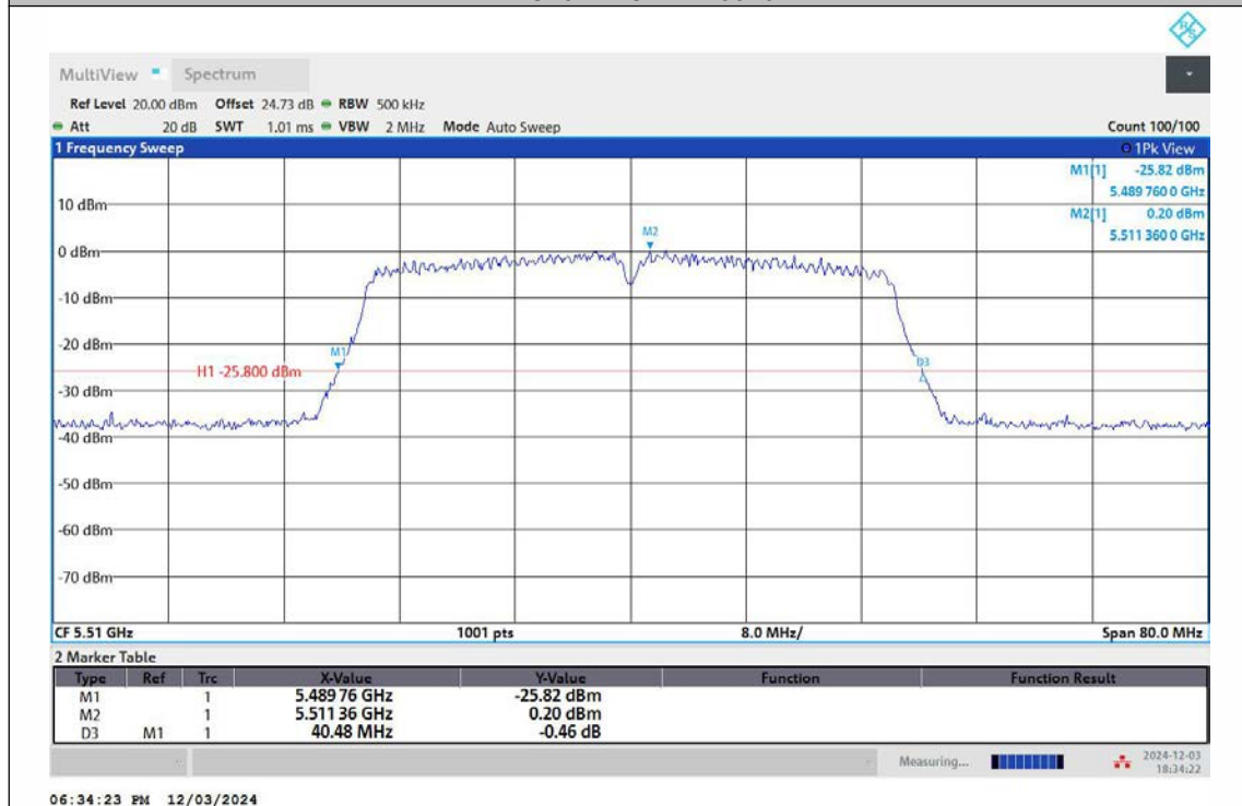
11AC40MIMO-Ant2-5510
