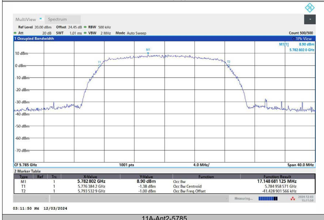
11A-Ant2-5785
