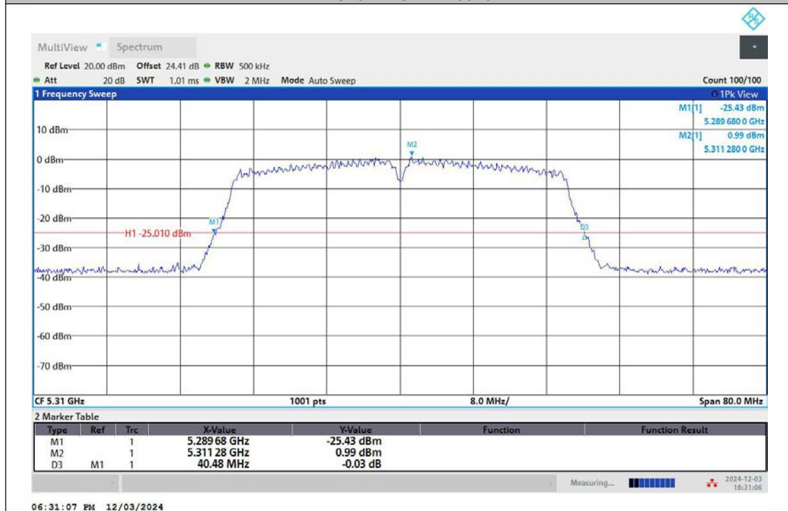
11AC40MIMO-Ant2-5310
