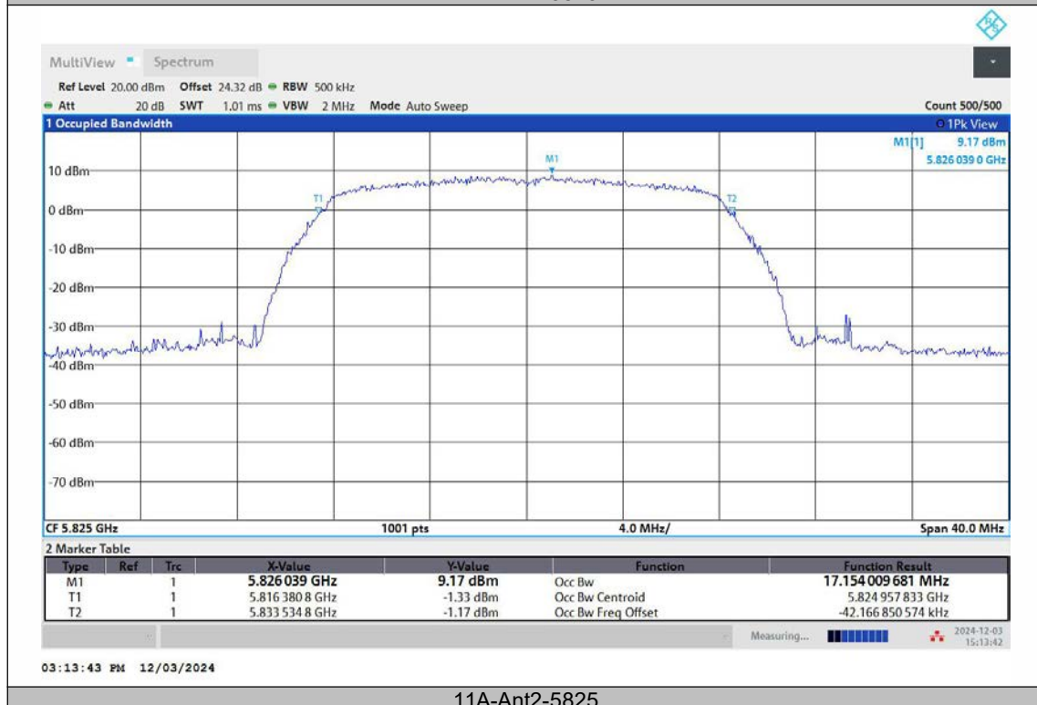
11A-Ant2-5825
