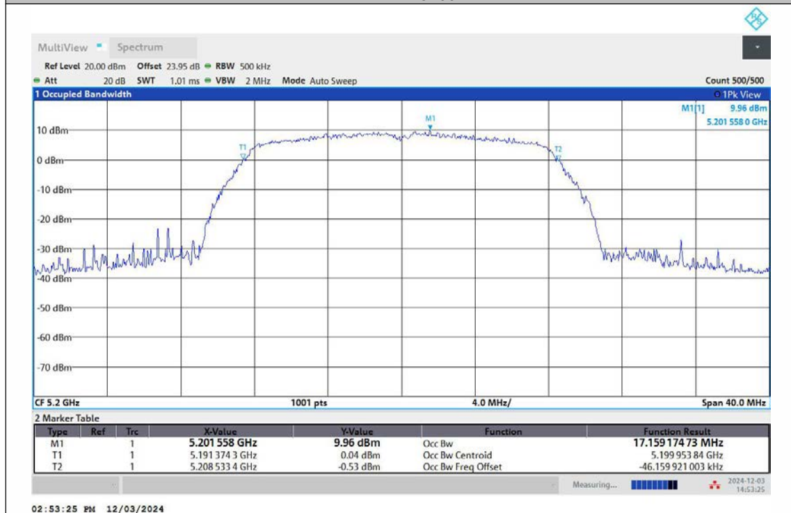
11A-Ant2-5200
