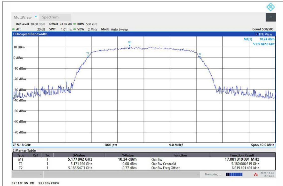
11A-Ant1-5180
