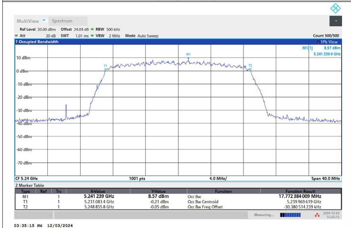
11N20MIMO-Ant2-5240
