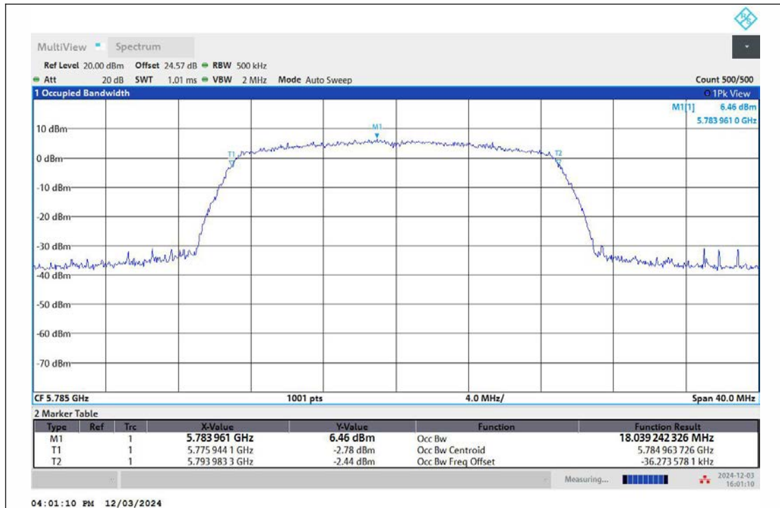
11N20MIMO-Ant1-5785
