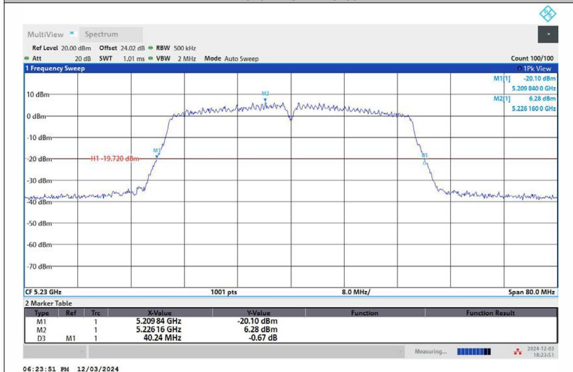
11AC40MIMO-Ant2-5230
