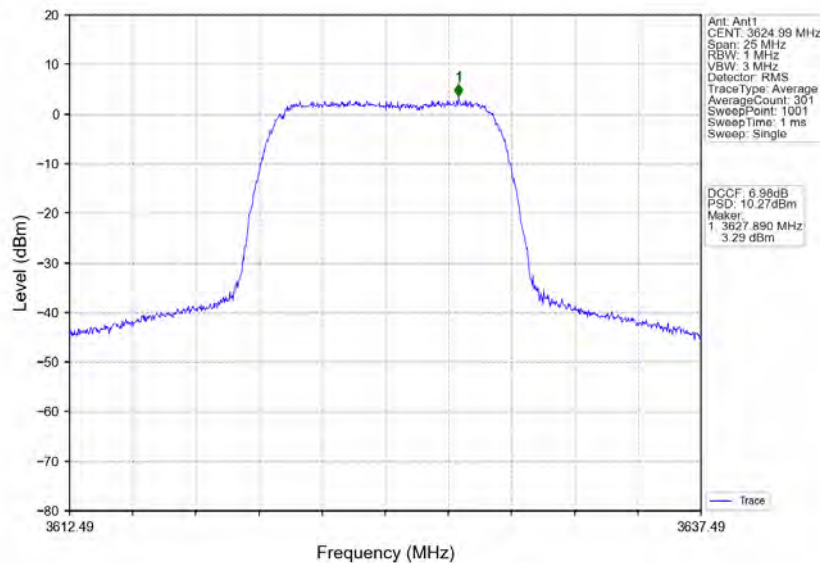
n48_30kHz_MIMO_NTNV_10MHz_CP-OFDM 16 QAM 3624.99MHz_Inner_Full
