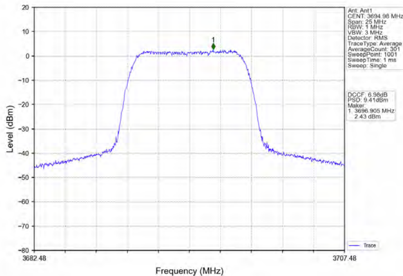
n48_30kHz_MIMO_NTNV_10MHz_CP-OFDM_16_QAM_3694.98MHz_Inner_Full
