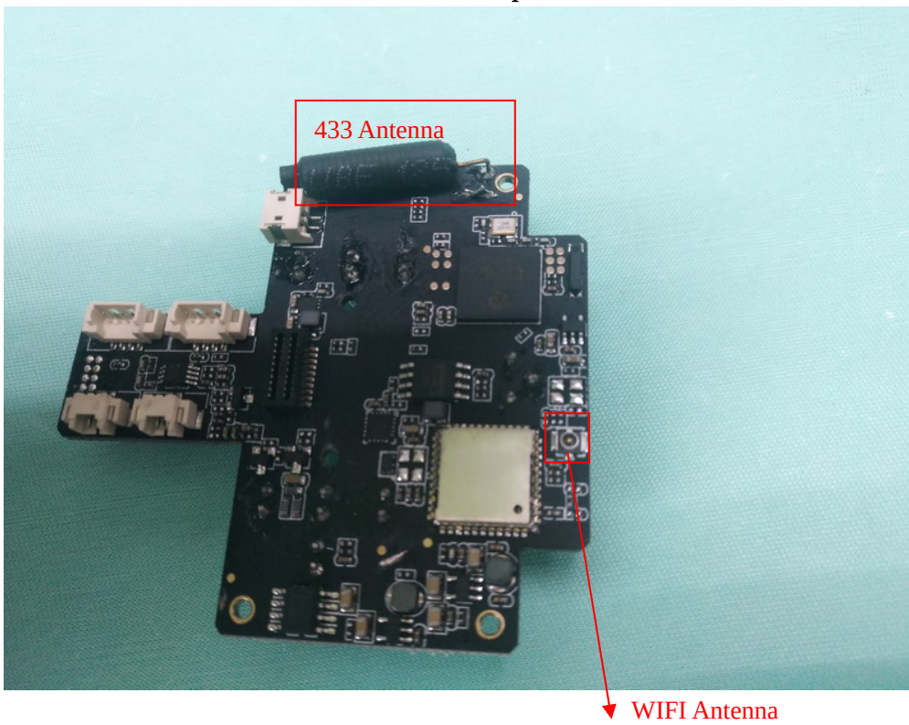
Inner Circuit Top View
