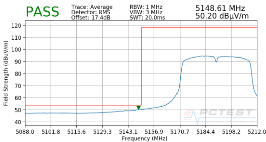
Plot 7-197. Radiated Lower Band Edge Plot SISO ANT2 (Average – UNII Band 1)
