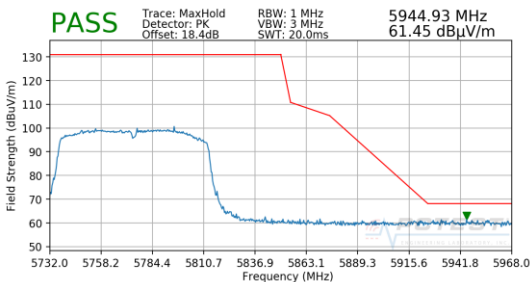
Plot 7-210. Radiated Upper Band Edge Plot SISO ANT2 (Peak – UNII Band 3)
