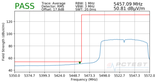
Plot 7-208. Radiated Lower Band Edge Plot SISO ANT2 (Average – UNII Band 2C)
