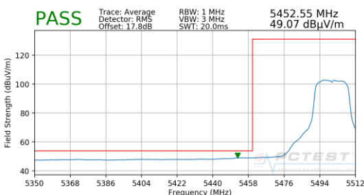
Plot 7-235. Radiated Lower Band Edge Plot MIMO (Average – UNII Band 2C)
