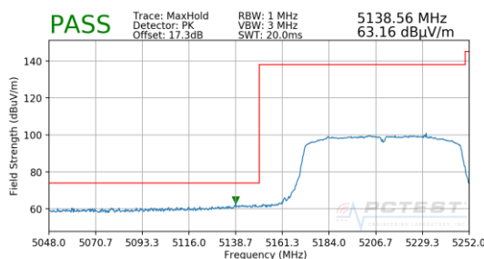
Plot 7-205. Radiated Lower Band Edge Plot SISO ANT2 (Peak – UNII Band 1)
