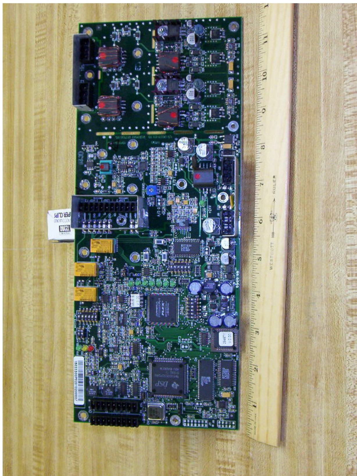
Photo 1 – Top Surface Detail of TR4025 Control PCB
