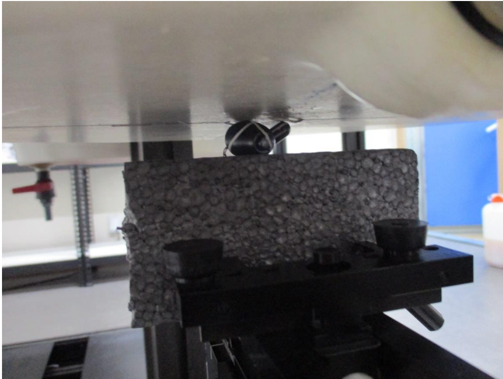
Right Side from Flat Phantom (Separation Distance: 0 cm) – Right Ear
