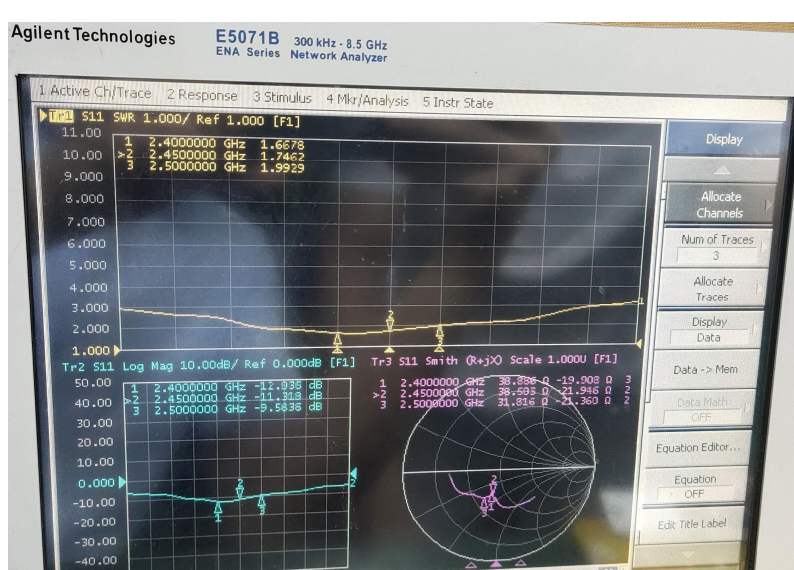
Test Photo:
