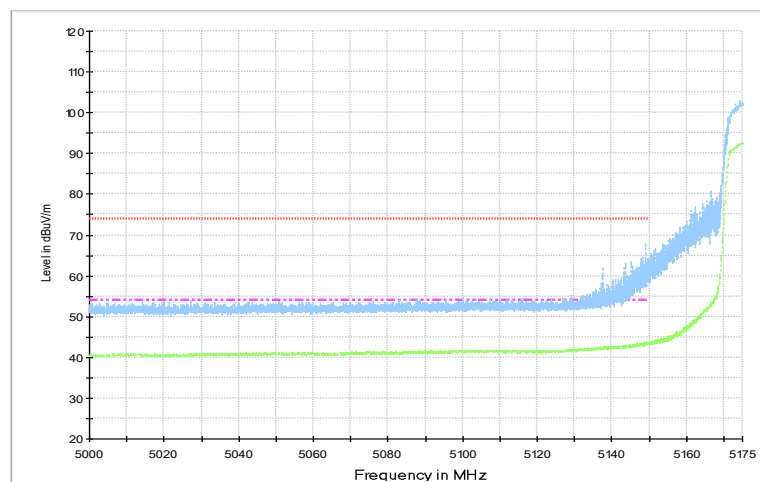
Fig.38 Band Edges (802.11n-HT20 Ch36, 5180MHz)
