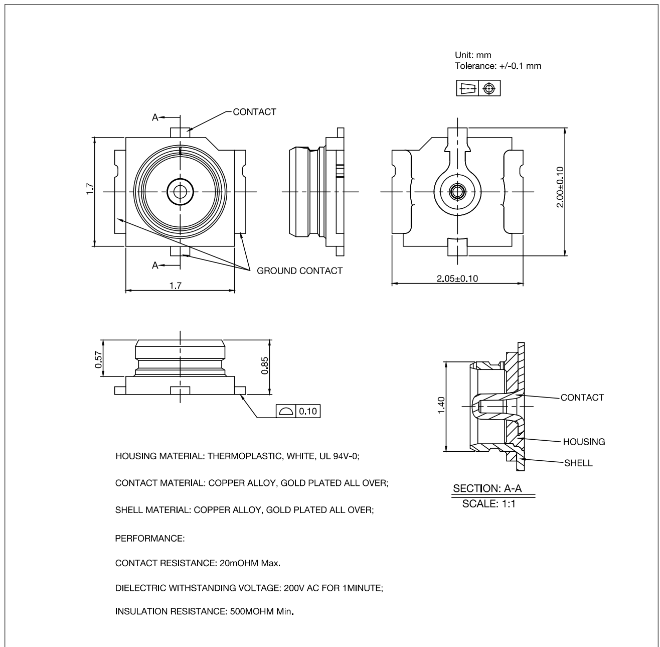
Figure 8: U.FL Connector Dimensions
