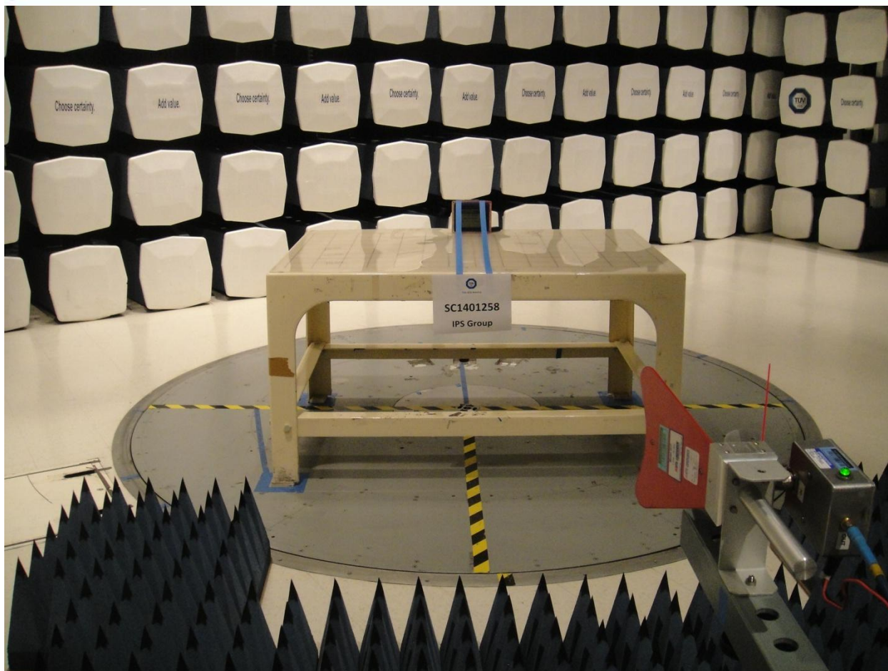
ISM/SRD Radiated Emission Measurement Above 1GHz (Front)
