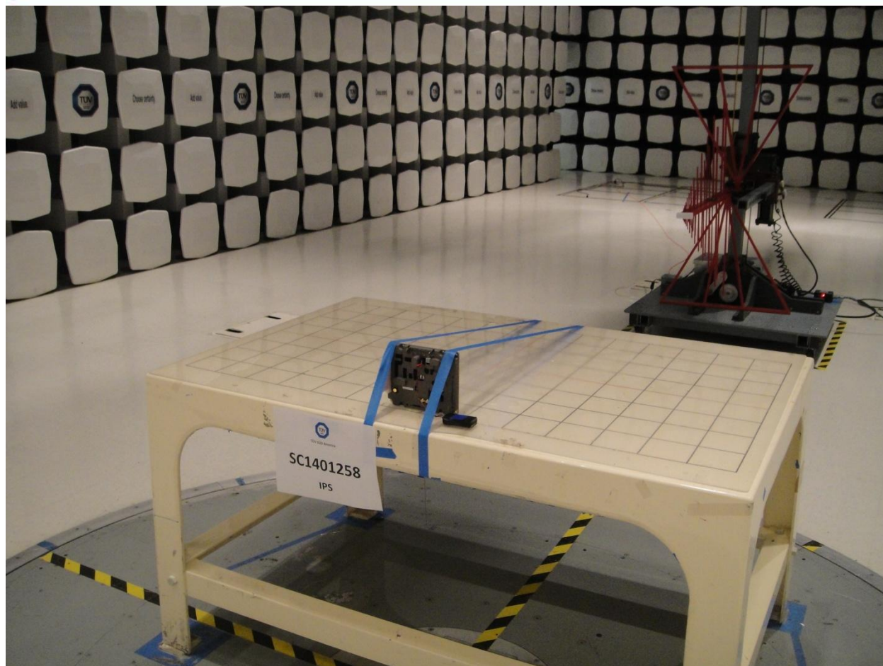
RFID and ISM/SRD Radiated Emission Measurement Below 1GHz (Back)
