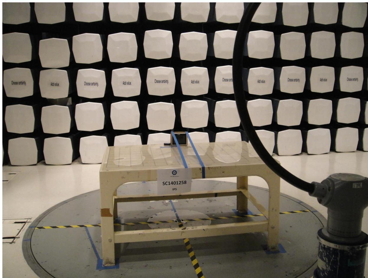
RFID Radiated Emission Measurement 9kHz to 30MHz (Front)
