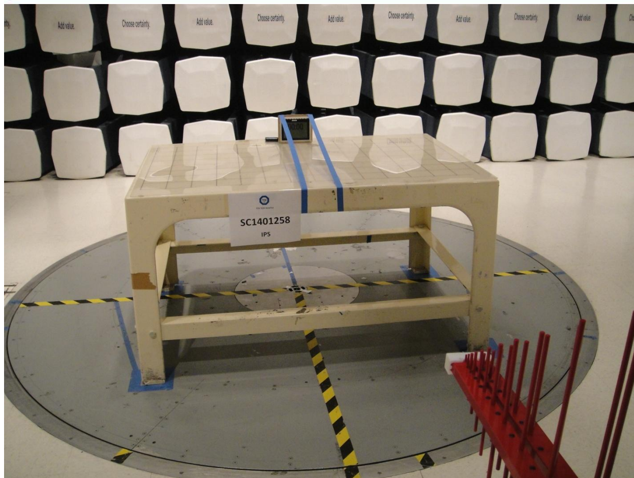
RFID and ISM/SRD Radiated Emission Measurement Below 1GHz (Front)
