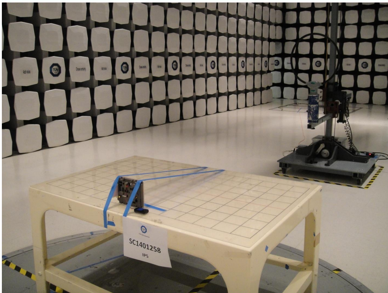
RFID Radiated Emission Measurement 9kHz to 30MHz (Back)
