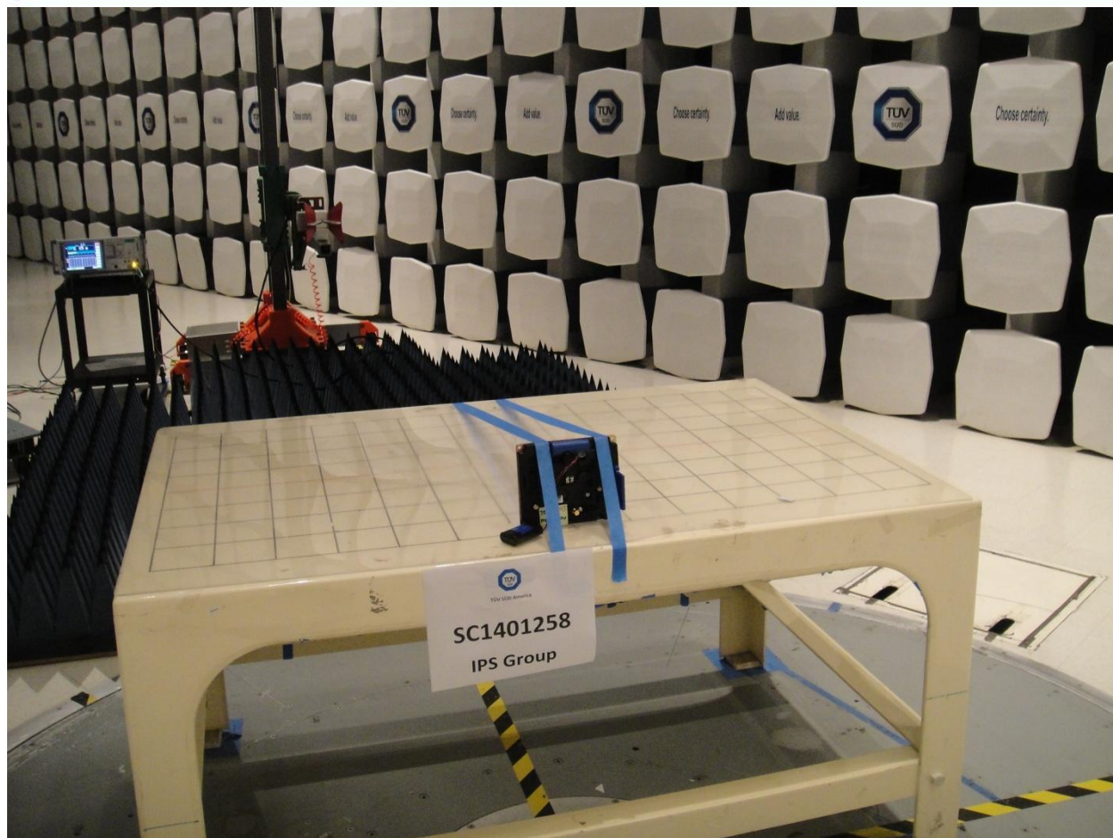
ISM/SRD Radiated Emission Measurement Above 1GHz (Back)
