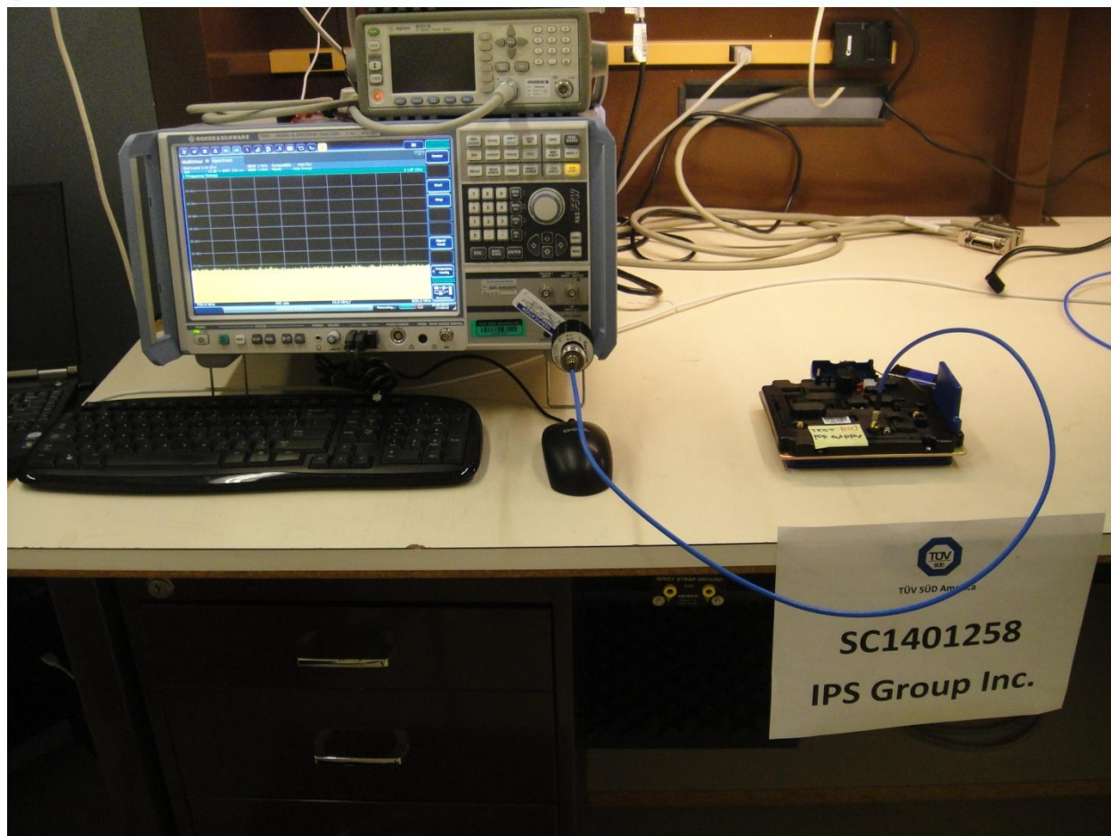
ISM/SRD Conducted Antenna Port Bandwidth Measurement
