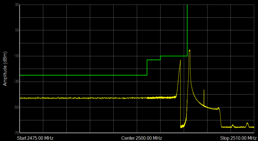
Band7 16QAM BW=5MHz Channel=20775 RB Size=1 Position=#0
