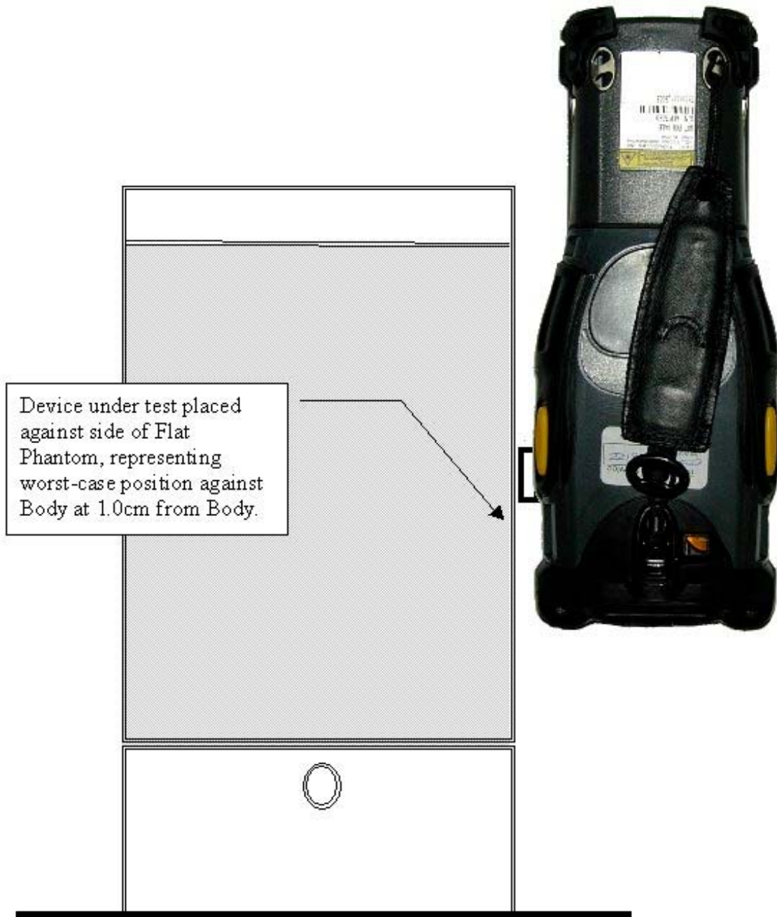
Figure 16. – MC9062 Test Position for WLAN Mode; 1.0 cm from phantom side (this does not represent the position of normal use but does give the maximum SAR level.)
