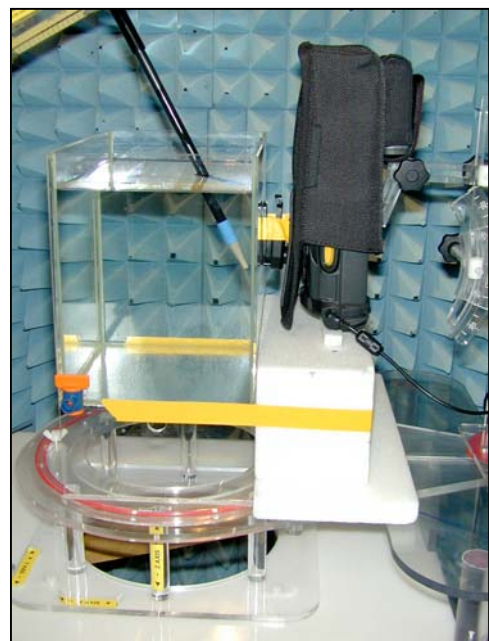
Figure 40. Positional photograph of the MC9062 With the device in a Mobile Computer Holster With the LCD side facing the rear of the Holster and the belt Clip in contact with the flat phantom.
