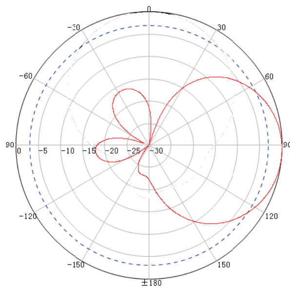
H Plane
