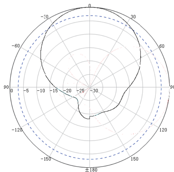
E Plane
