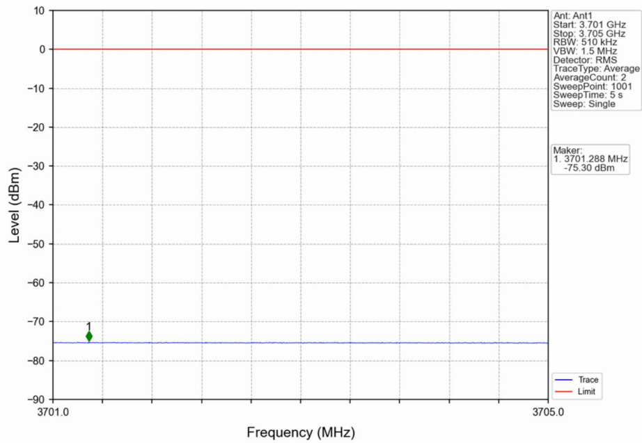
n48_30kHz_SISO_NTNV_10MHz_CP-OFDM QPSK_3694.98MHz_Outer_Full
