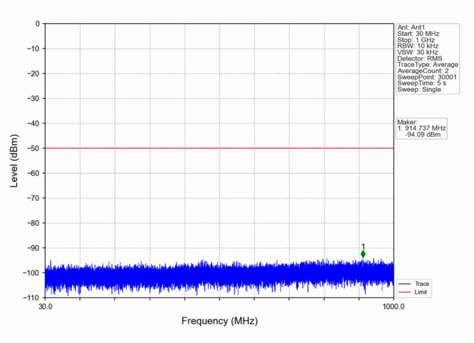
n48_30kHz_SISO_NTNV_10MHz_CP-OFDM QPSK_3694.98MHz_Outer_Full
