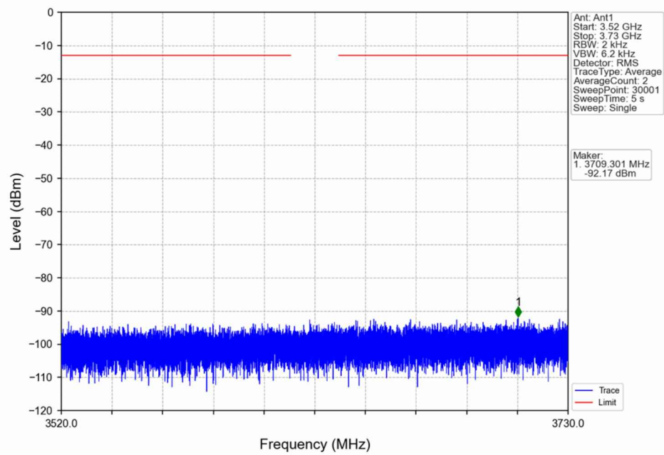
n48_30kHz_SISO_NTNV_20MHz_DFT-s-OFDM QPSK_3624.99MHz_Edge_1RB_Left
