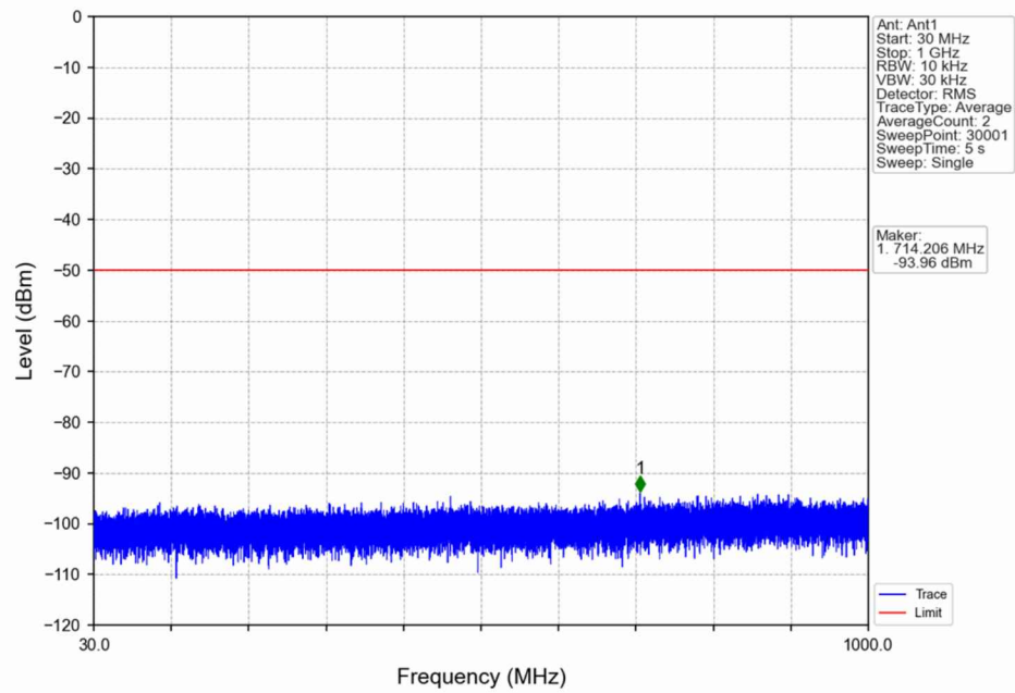
n48_30kHz_SISO_NTNV_10MHz_CP-OFDM QPSK_3694.98MHz_Edge_1RB_Right
