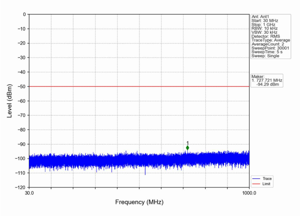
n48_30kHz_SISO_NTNV_20MHz_DFT-s-OFDM QPSK_3560.01MHz_Outer_Full
