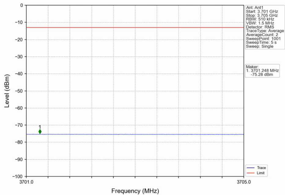
n48_30kHz_SISO_NTNV_10MHz_CP-OFDM QPSK_3694.98MHz_Inner_1RB_Right
