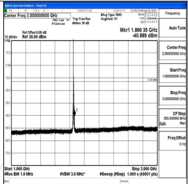
Band2_5MHz_QPSK_18625_1RB#0_1000~3000_1000~3000
