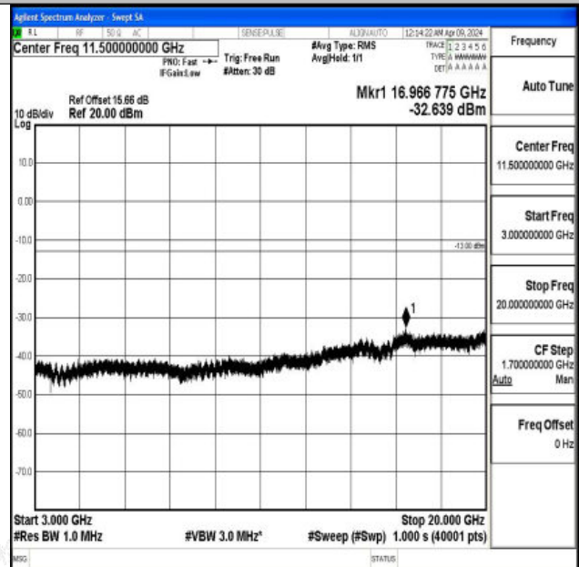
Band2_3MHz_16QAM_19185_1RB#0_3000~20000_3000~20000
