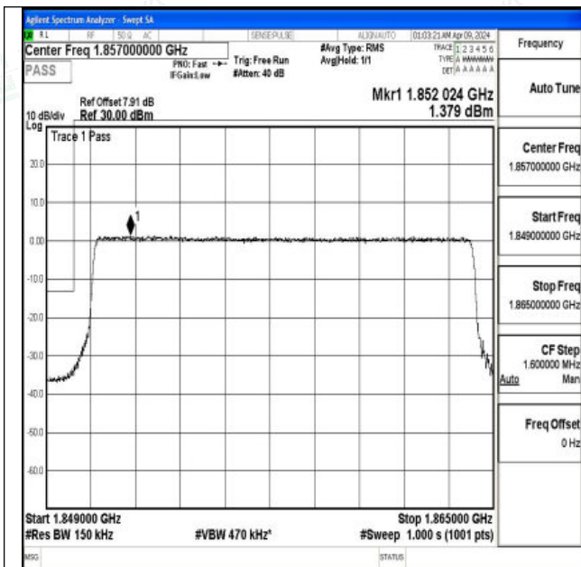
Band2_15MHz_QPSK_18675_75RB#0
