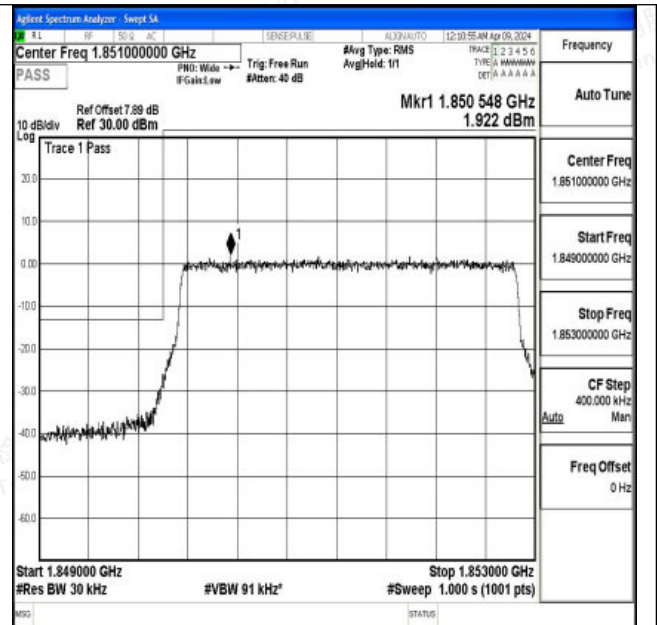
Band2_3MHz_16QAM_18615_15RB#0
