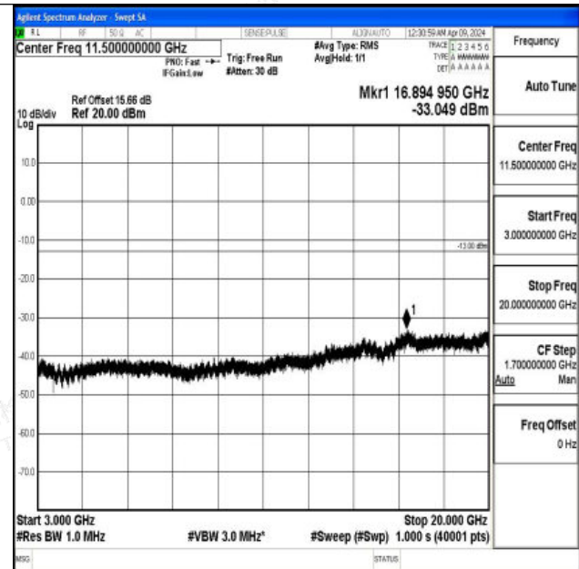
Band2_5MHz_16QAM_18625_1RB#0_3000~20000_3000~20000
