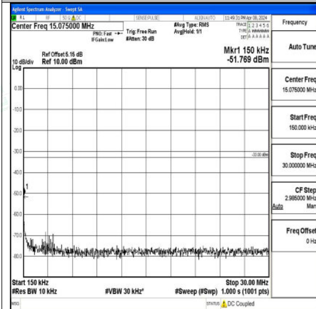
Band2_1.4MHz_16QAM_19193_1RB#0_0.15~30_0.15~30
