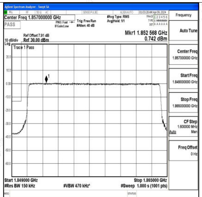
Band2_15MHz_16QAM_18675_75RB#0
