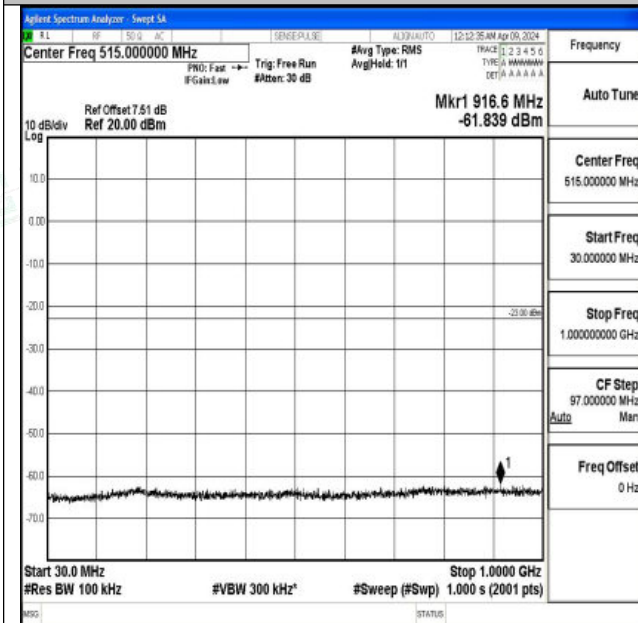
Band2_3MHz_QPSK_18900_1RB#0_30~1000_30~1000
