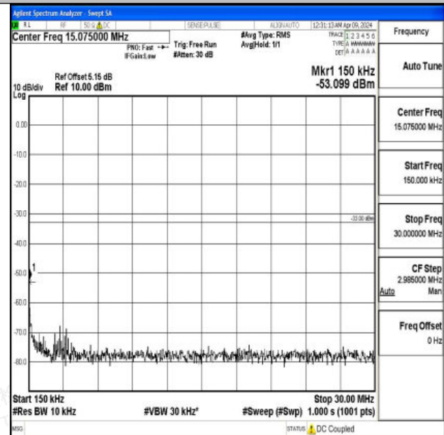
Band2_5MHz_QPSK_18900_1RB#0_0.15~30_0.15~30
