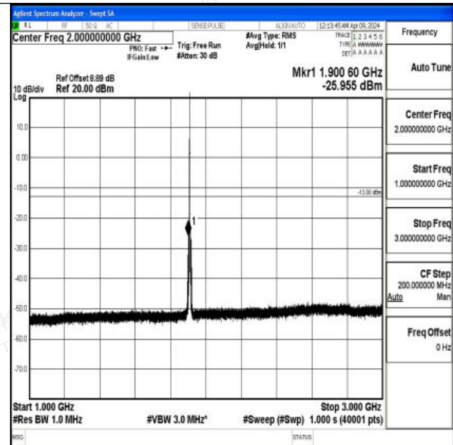
Band2_3MHz_QPSK_19185_1RB#0_1000~3000_1000~3000
