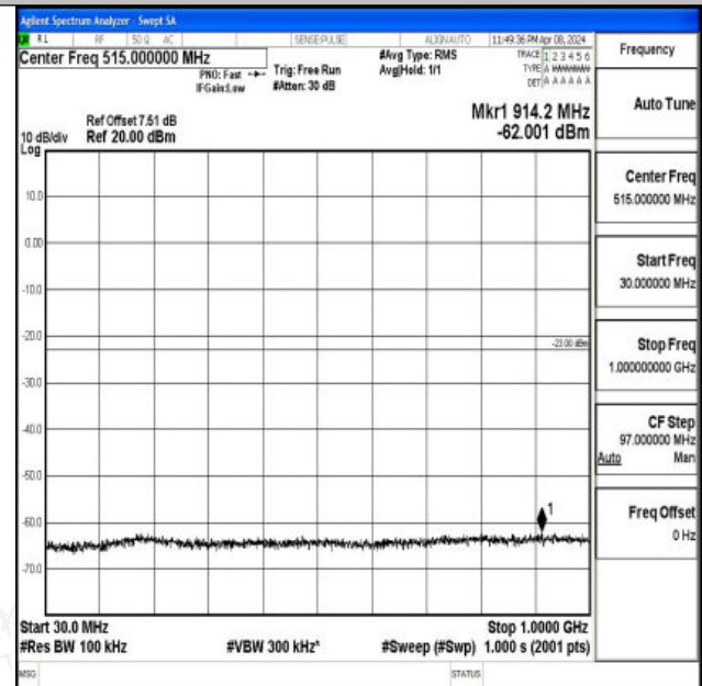
Band2_1.4MHz_16QAM_19193_1RB#0_30~1000_30~1000
