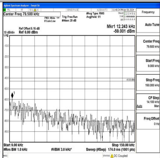
Band2_1.4MHz_16QAM_18900_1RB#0_0.009~0.15_0.009~0.15
