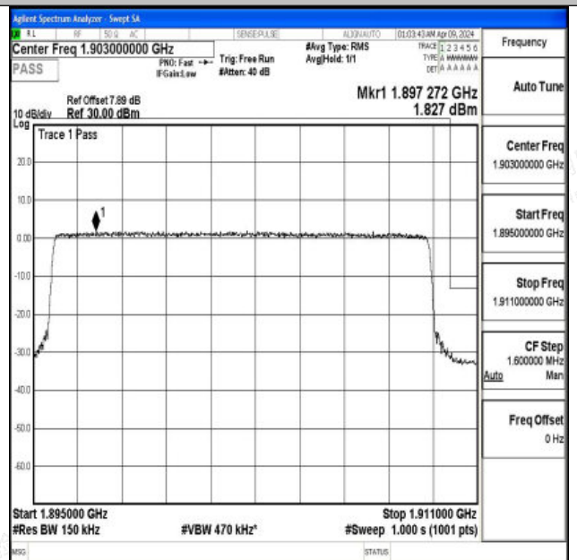
Band2_15MHz_16QAM_19125_75RB#0
