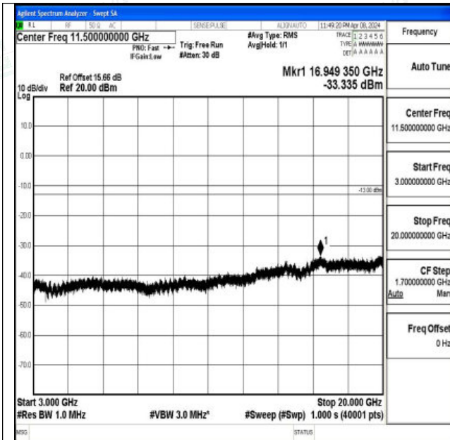
Band2_1.4MHz_QPSK_19193_1RB#0_3000~20000_3000~20000
