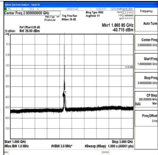
Band2_5MHz_QPSK_18900_1RB#0_1000~3000_1000~3000
