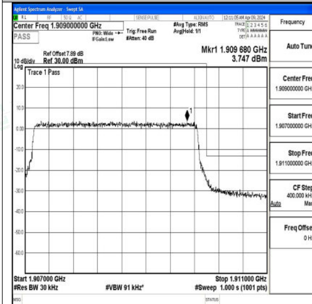
Band2_3MHz_QPSK_19185_15RB#0
