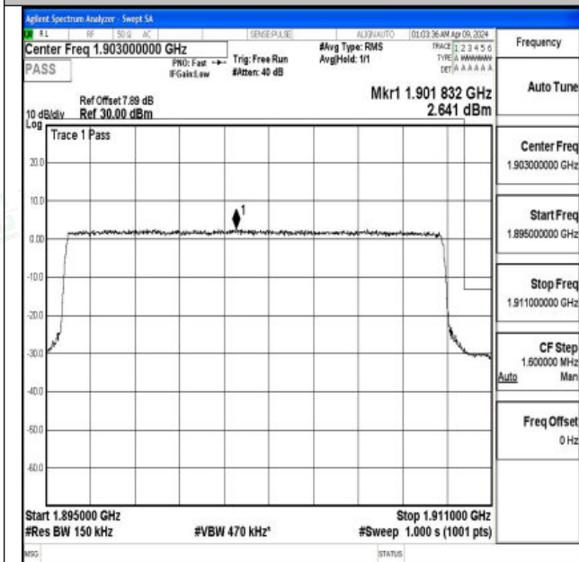
Band2_15MHz_QPSK_19125_75RB#0
