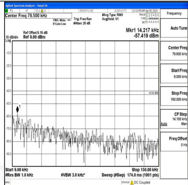
Band2_3MHz_16QAM_19185_1RB#0_0.009~0.15_0.009~0.15
