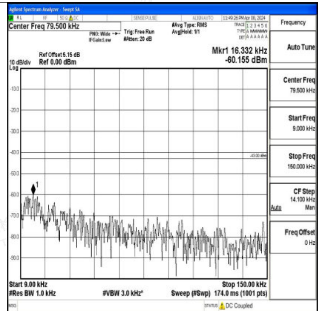
Band2_1.4MHz_16QAM_19193_1RB#0_0.009~0.15_0.009~0.15
