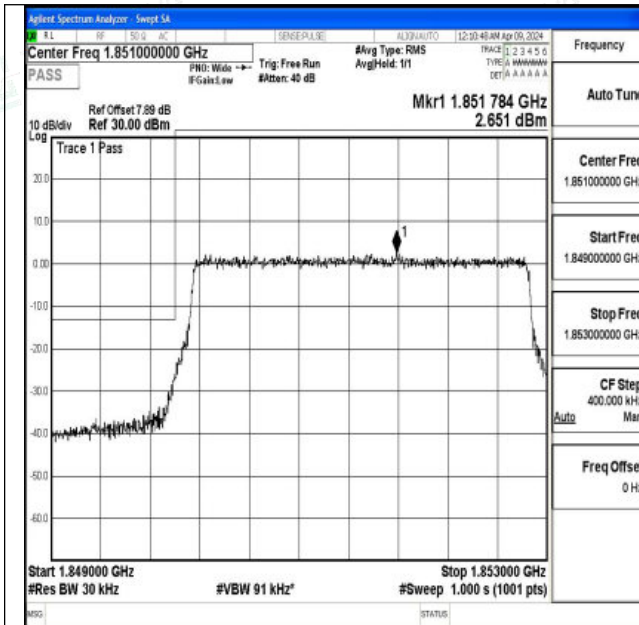
Band2_3MHz_QPSK_18615_15RB#0
