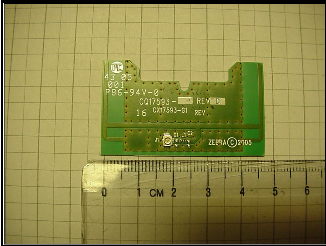
Photograph 3: Top of Antenna CQ17593-G1
