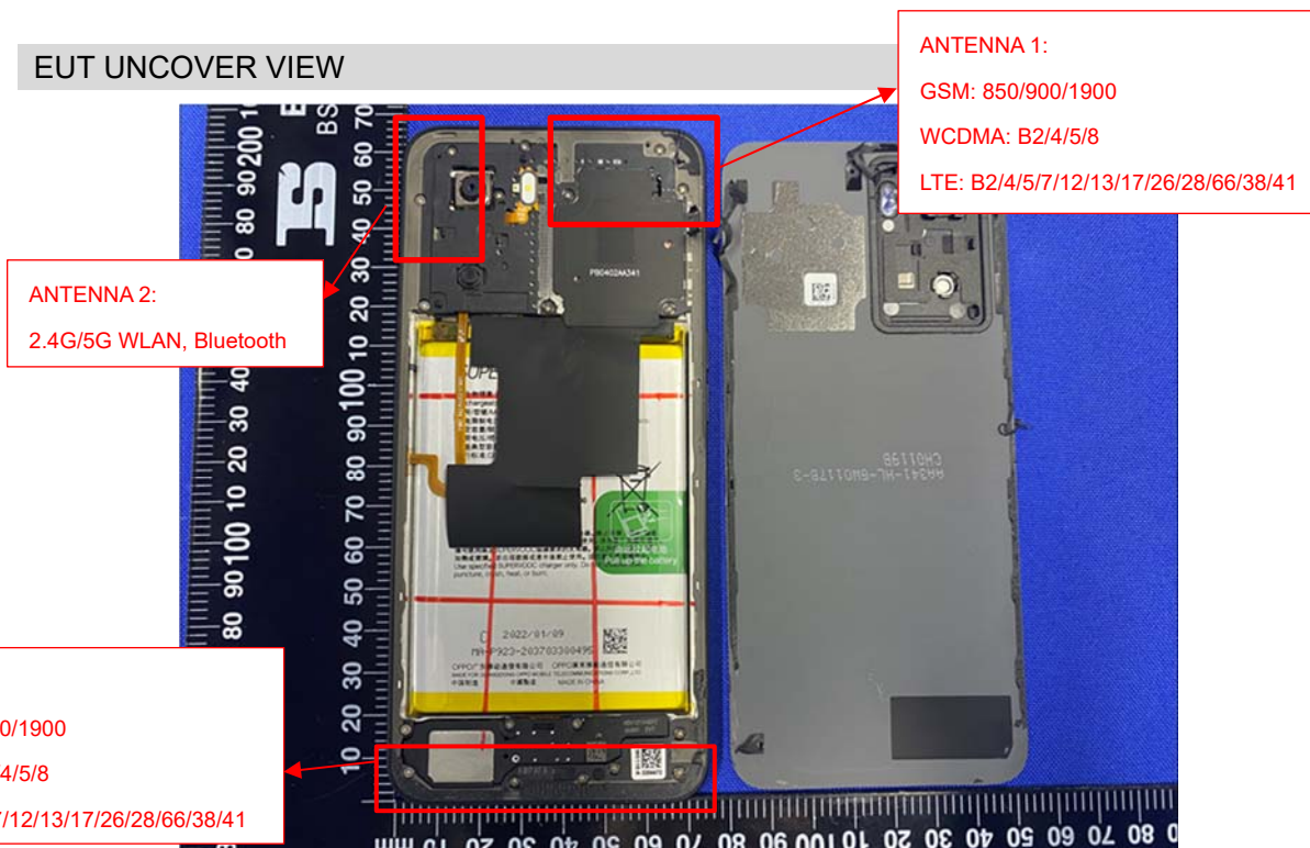
EUT UNCOVER VIEW
