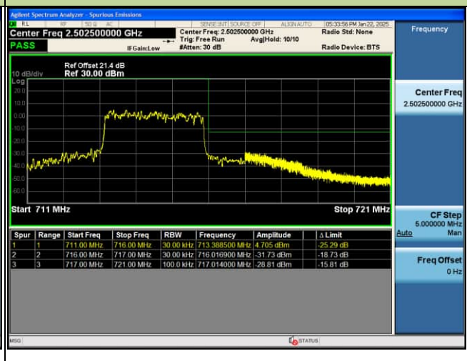
EDGE_4G_B12_16QAM_3M_FULLRB@MAX_CH23165
