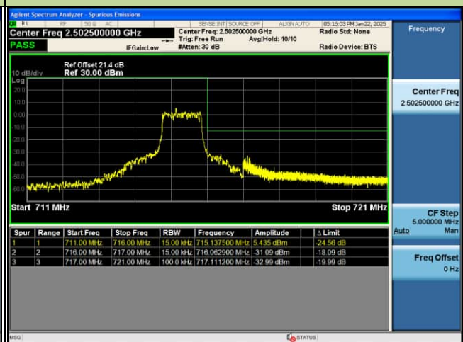
EDGE_4G_B12_64QAM_1.4M_FULLRB@MAX_CH23173
