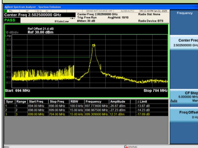
EDGE_4G_B12_16QAM_1.4M_1RB@0_CH23017
