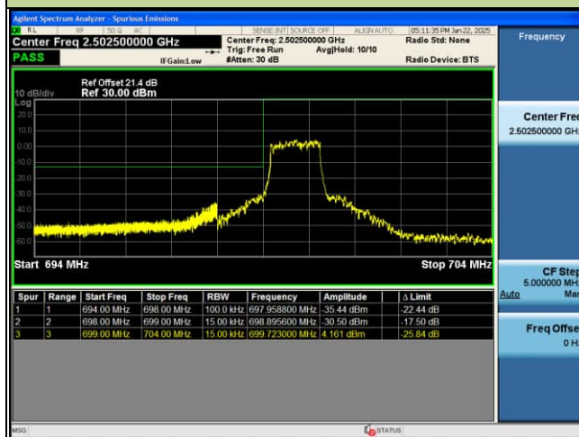
EDGE_4G_B12_16QAM_1.4M_FULL_RB@0_CH23017
