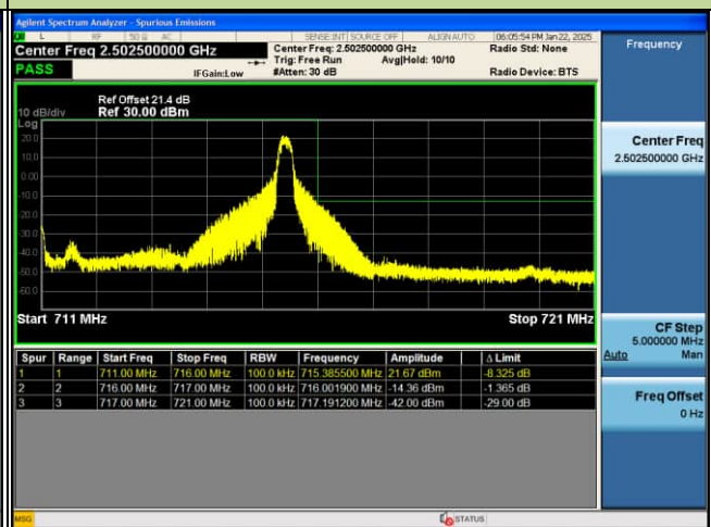
EDGE_4G_B12_QPSK_10M_1RB@MAX_CH23130
