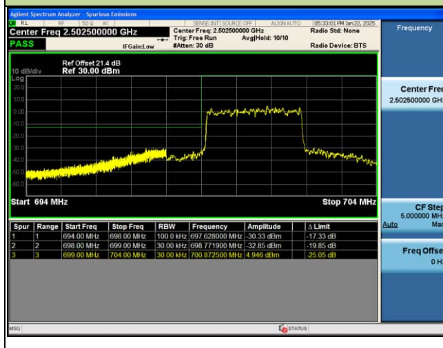
EDGE_4G_B12_16QAM_3M_FULL RB@0_CH23025
