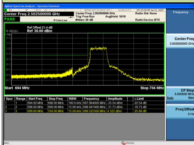
EDGE_4G_B12_64QAM_1.4M_FULL RB@0_CH23017
