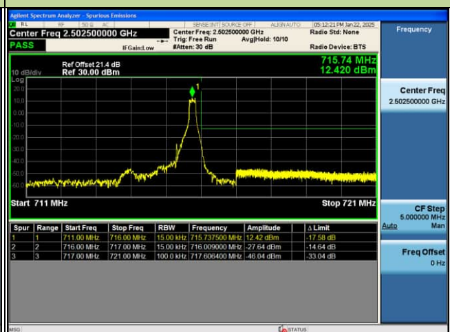
EDGE_4G_B12_16QAM_1.4M_1RB@MAX_CH23173
