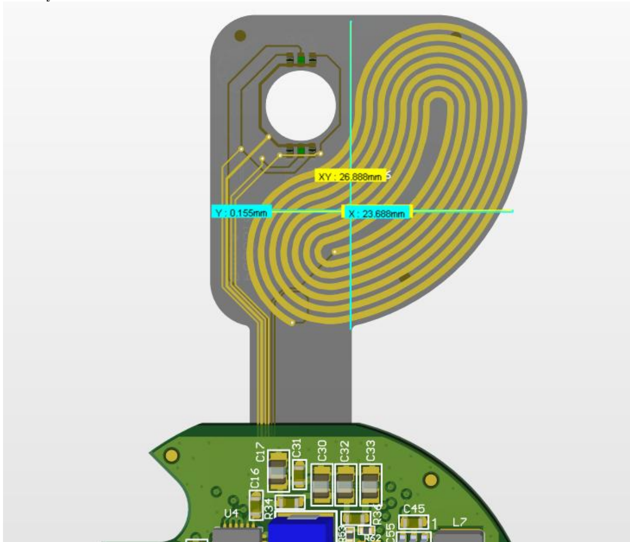
NFC layout in 3D
