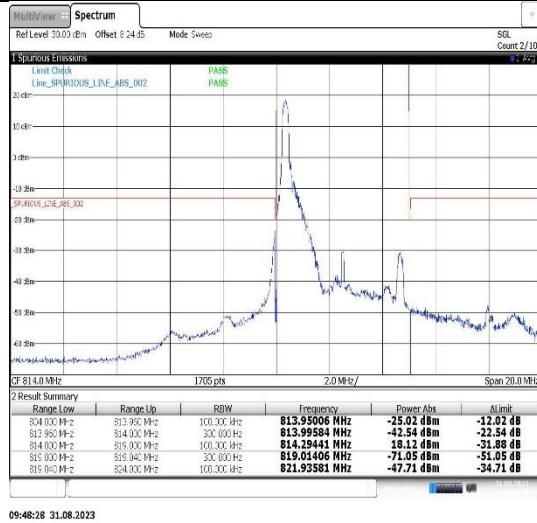
Band26(814-824)-5MHz-16QAM-26765-1RB#24
