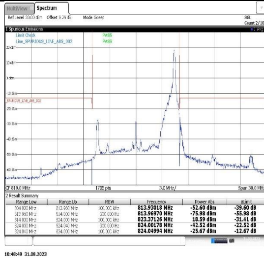
Band26(824-849)-1.4MHz-QPSK-26797-1RB#0
