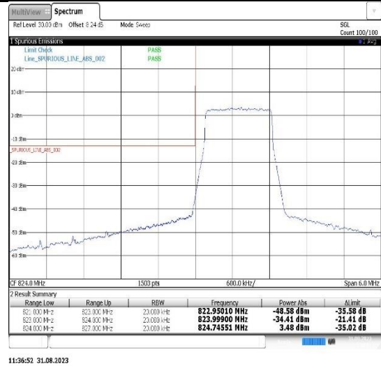
Band26(824-849)-1.4MHz-16QAM-27033-6RB#0
