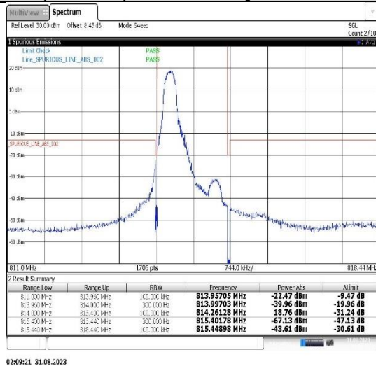
Band26(814-824)-1.4MHz-16QAM-26783-1RB#5
