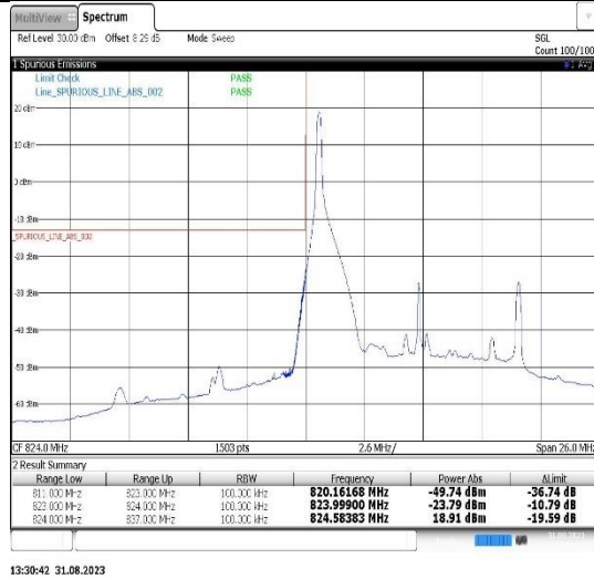
Band26(824-849)-10MHz-16QAM-26840-1RB#0
