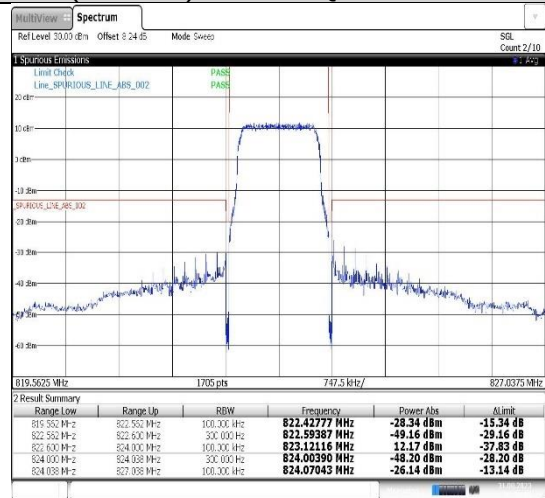
Band26(814-824)-1.4MHz-QPSK-26783-6RB#0
