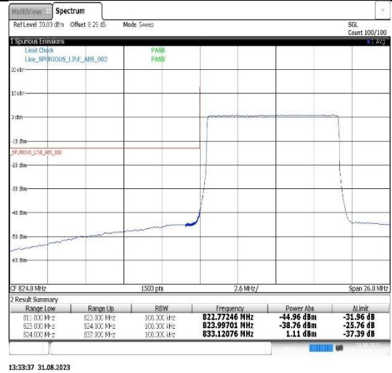
Band26(824-849)-15MHz-QPSK-26865-75RB#0
