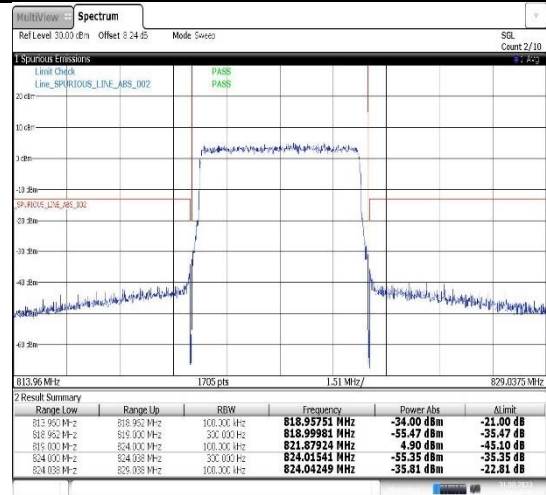
Band26(814-824)-10MHz-QPSK-26740-1RB#49
