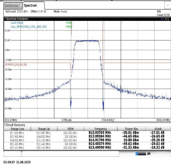
Band26(814-824)-1.4MHz-16QAM-26783-6RB#0
