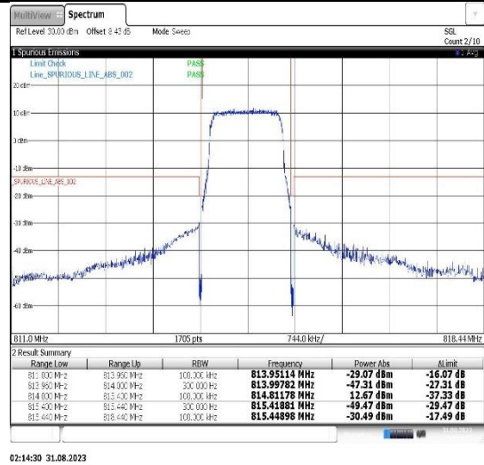
Band26(814-824)-1.4MHz-QPSK-26783-6RB#0
