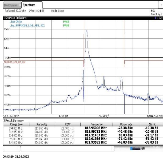
Band26(814-824)-5MHz-QPSK-26765-1RB#24
