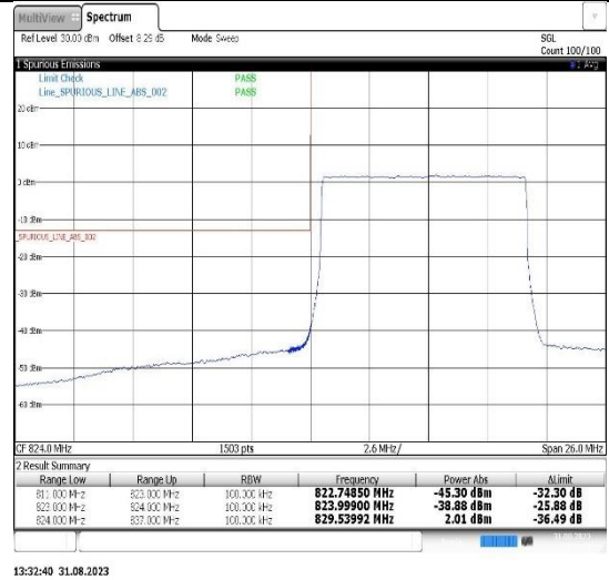
Band26(824-849)-10MHz-16QAM-26840-50RB#0
