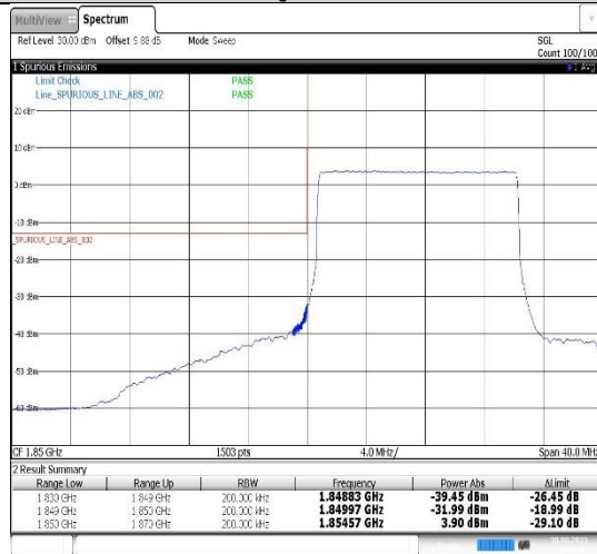
Band25-15MHz-QPSK-26115-75RB#0
