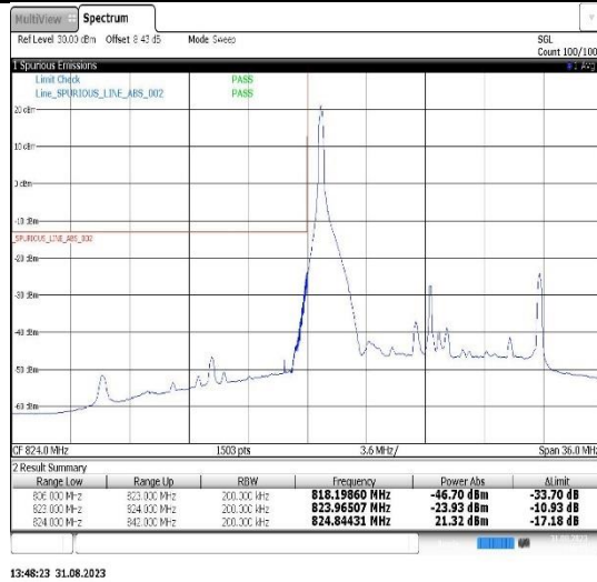
Band26(824-849)-15MHz-16QAM-26865-1RB#0
