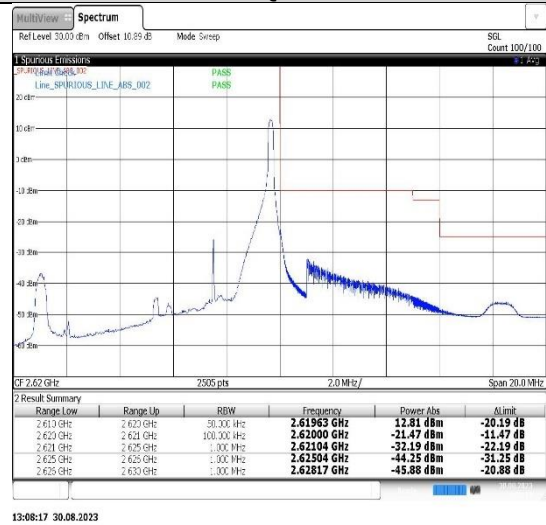
Band38-10MHz-QPSK-37800-1RB#0
