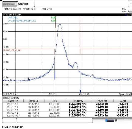
Band26(814-824)-1.4MHz-QPSK-26783-1RB#5
