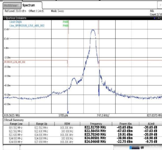
Band26(814-824)-1.4MHz-QPSK-26783-1RB#5
