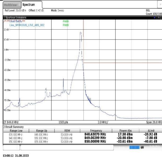
Band26(824-849)-5MHz-16QAM-26815-1RB#0
