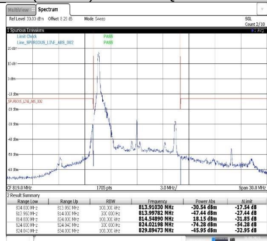
Band26(814-824)-10MHz-16QAM-26740-1RB#0
