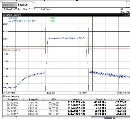
Band26(814-824)-10MHz-QPSK-26740-50RB#0
