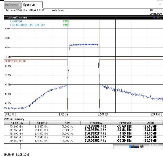
Band26(814-824)-5MHz-16QAM-26765-25RB#0
