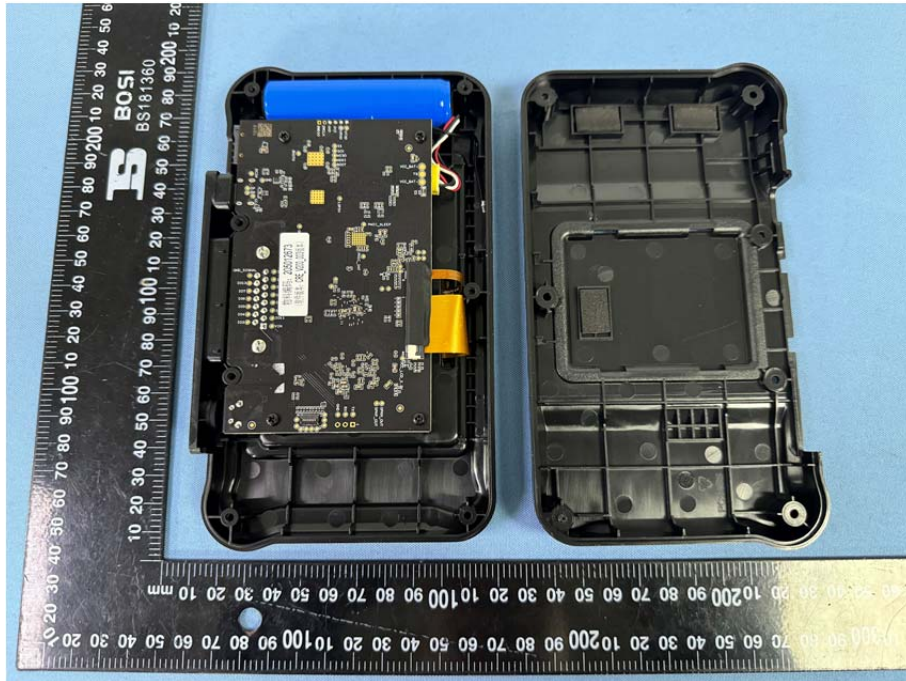
OCE-X403A Internal Photographs
