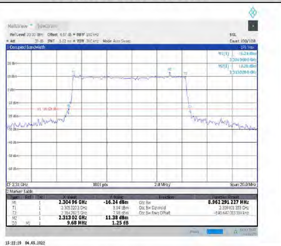
1-N30--15-10-H-3-DFT-16QAM-Outer_Full-50@0-Ant1-8.962-9.680-≤10-PASS
