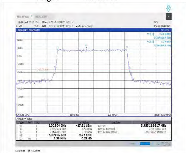
1-N30--15-10-H-5-DFT-256QAM-Outer_Full-50@0-Ant1-8.955-9.580-≤10-PASS
