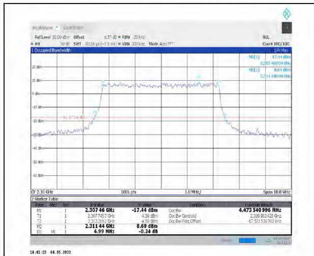
1-N30--15-5-M-8-CP-64QAM-Outer_Full-25@0-Ant1-4.474-4.990-≤5-PASS
