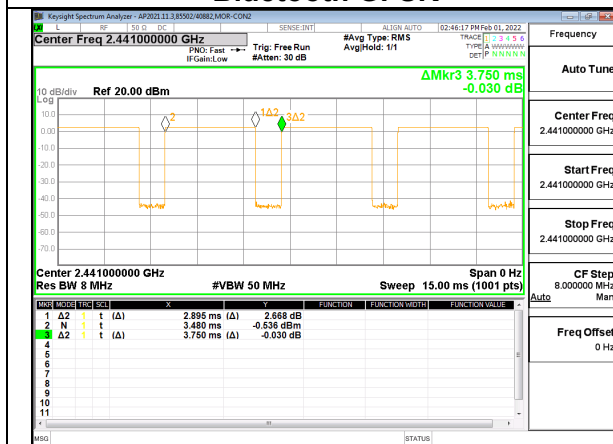
Bluetooth GFSK
