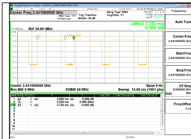
Bluetooth GFSK
