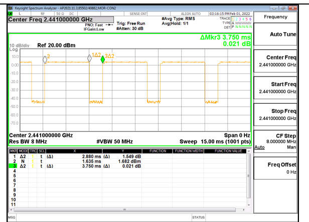
Bluetooth 8PSK
