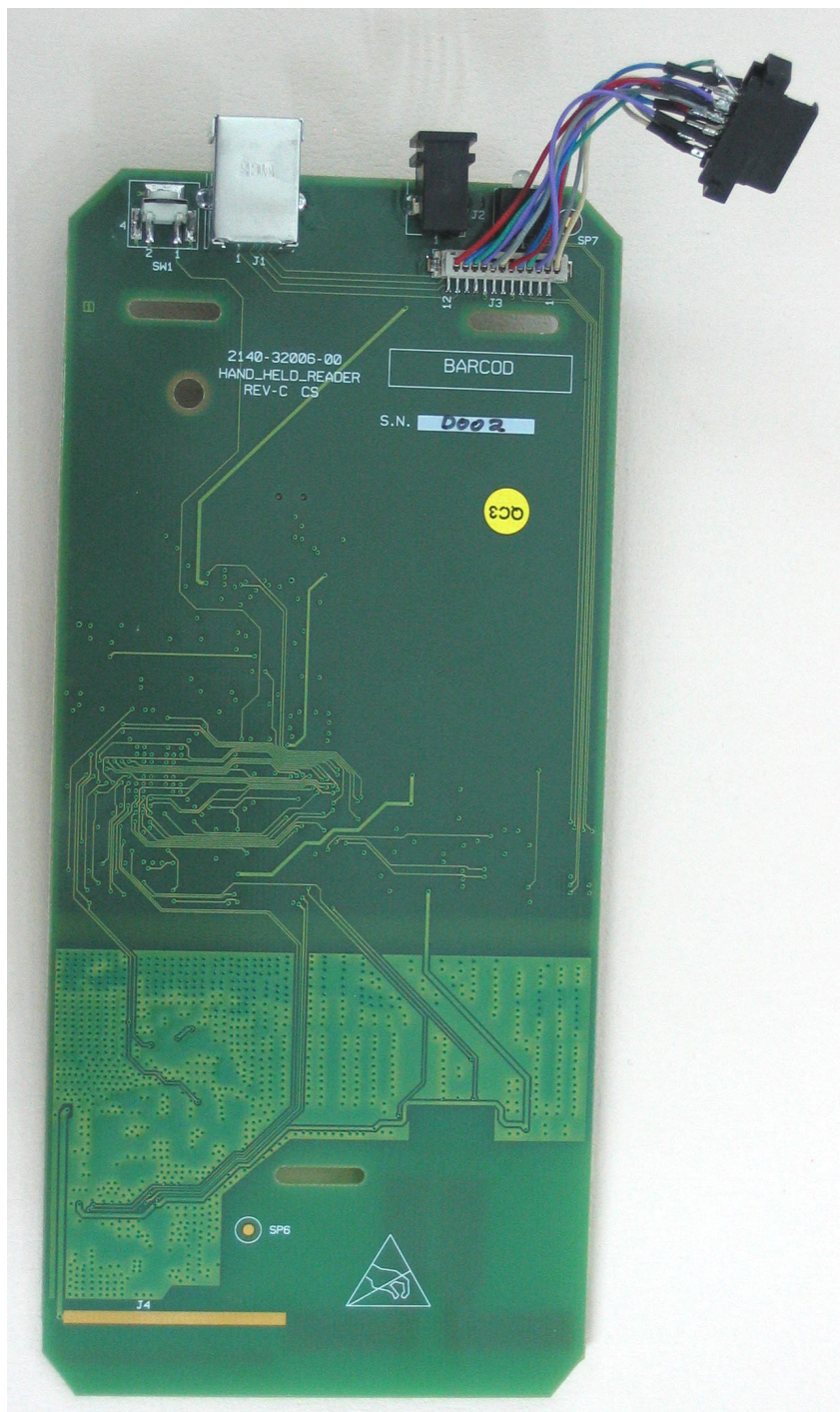
Photograph No.4 FP200HH handheld reader PCB second side view
