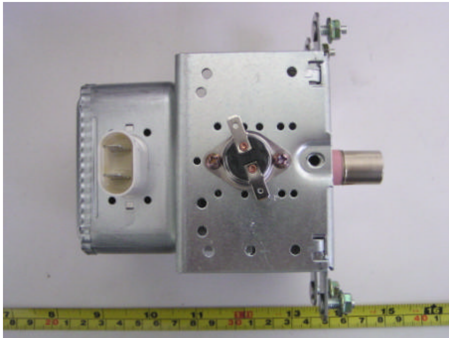
EUT- Magnetism Signal Generator View
