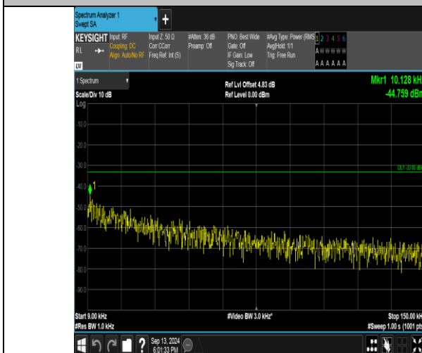
Band26_10MHz_QPSK_26740_1RB#49_0.009~0.15_0.009~0.15
