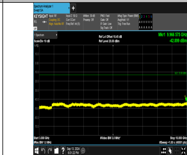
Band26_10MHz_16QAM_26740_1RB#0_3000~10000_3000~10000
