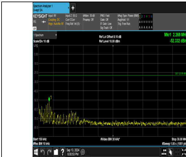
Band26_10MHz_16QAM_26740_1RB#0_0.15~30_0.15~30
