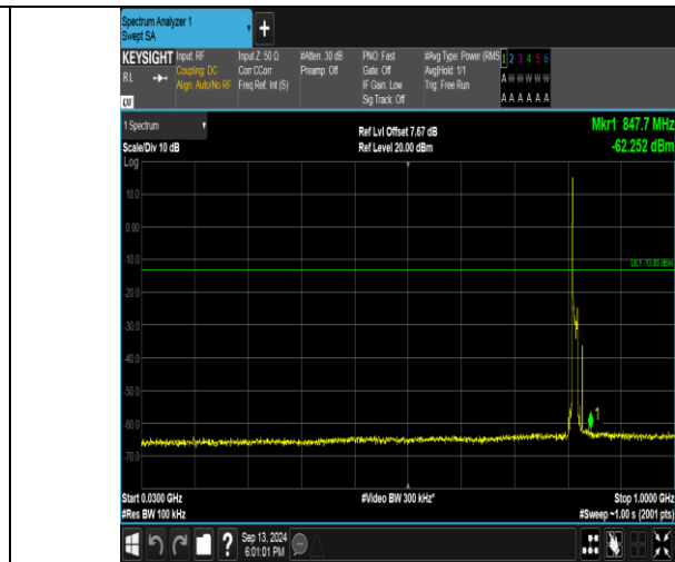
Band26_10MHz_16QAM_26740_1RB#0_30~1000_30~1000
