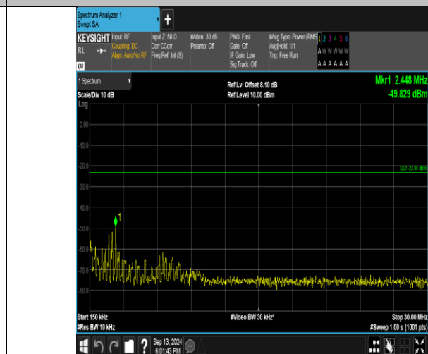
Band26_10MHz_QPSK_26740_1RB#49_0.15~30_0.15~30
