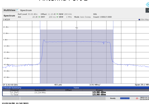
Antenna Port 2
