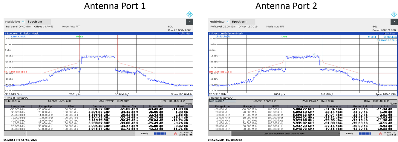
Figure 4.3.2 (i) Worst Case Transmitter OOBE Emissions Measured.
