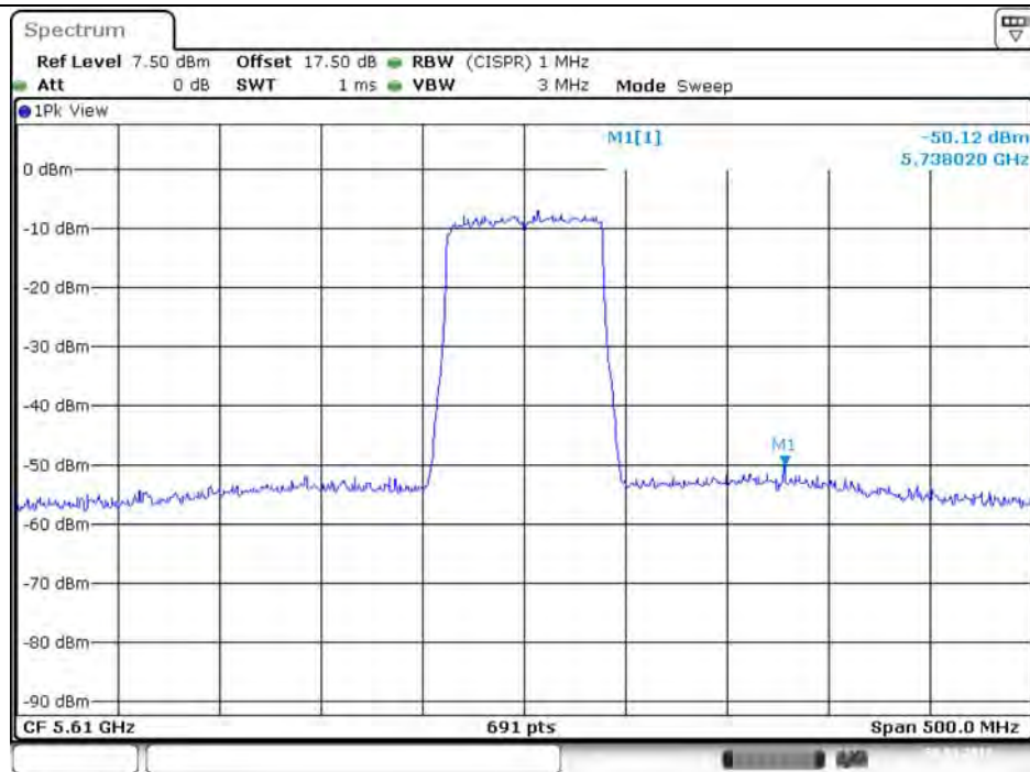
Plot on Configuration VHT80 / 5610 MHz / Peak / Port 1
