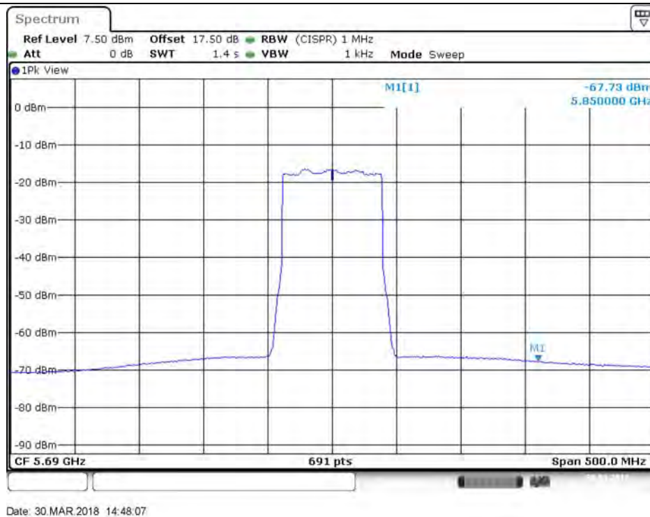
Plot on Configuration VHT80 / 5690 MHz / Average / Port 2
