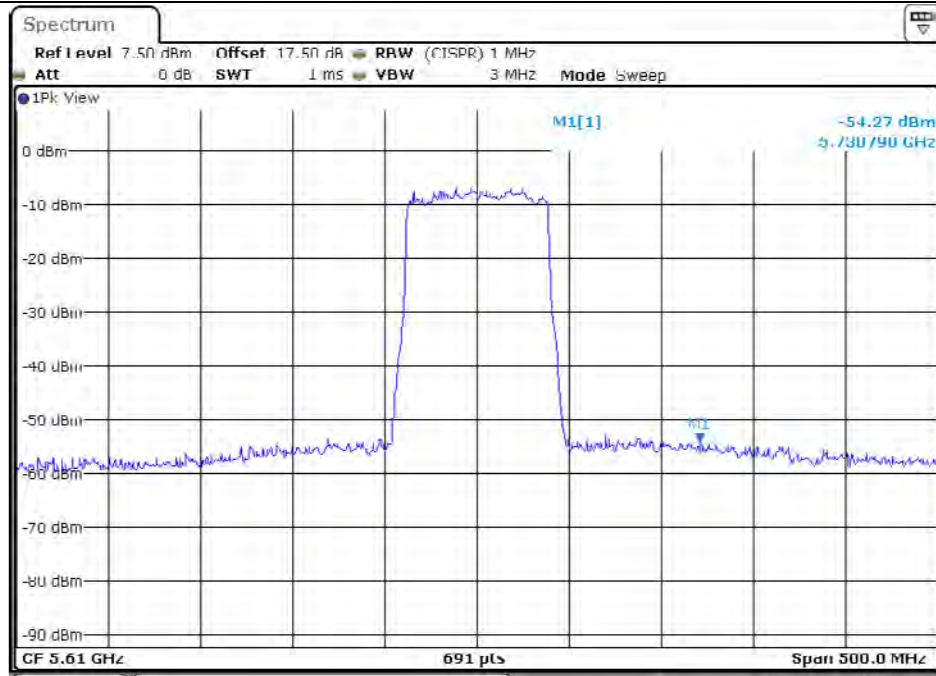
Plot on Configuration VHT80 / 5610 MHz / Peak / Port 2
