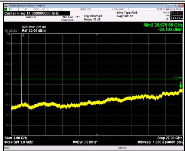
41-41-5MHz-20MHz-64QAM-64QAM-40528-40645-1RB#0-0RB#0-1000~27000MHz-PASS
