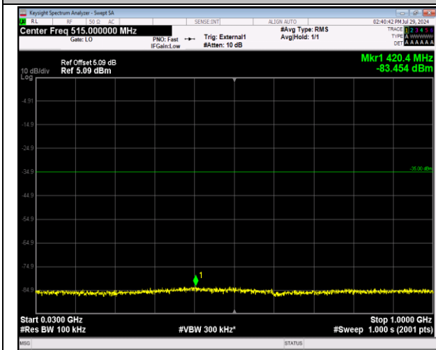
41-41-5MHz-20MHz-64QAM-64QAM-40528-40645-25RB #0-100RB#0-30~1000MHz-PASS
