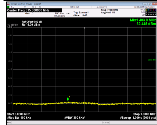
41-41-5MHz-20MHz-64QAM-64QAM-40528-40645-1RB# 24-ORB#0-30~1000MHz-PASS
