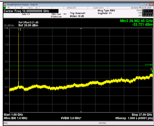
41-41-5MHz-20MHz-64QAM-64QAM-41373-41490-1RB#0- 0RB#0-1000~27000MHz-PASS
