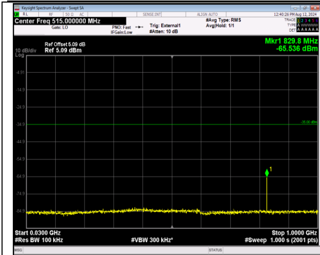
41-41-5MHz-20MHz-16QAM-16QAM-39683-39800-25RB #0-100RB#0-30~1000MHz-PASS
