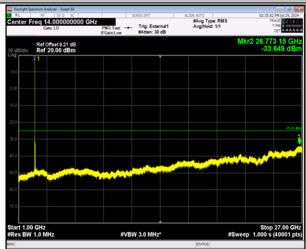
41-41-5MHz-20MHz-64QAM-64QAM-39683-39800-1RB#0- 0RB#0-1000~27000MHz-PASS
