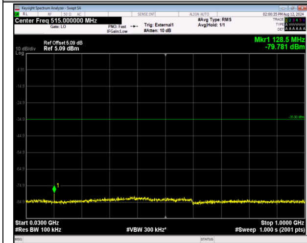
41-41-20MHz-5MHz-QPSK-QPSK-39750-39867-1RB#0-0 ORB#0-30~1000MHz-PASS
