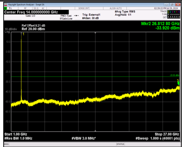
41-41-5MHz-20MHz-64QAM-64QAM-40528-40645-1RB#24 -ORB#0-1000~27000MHz-PASS
