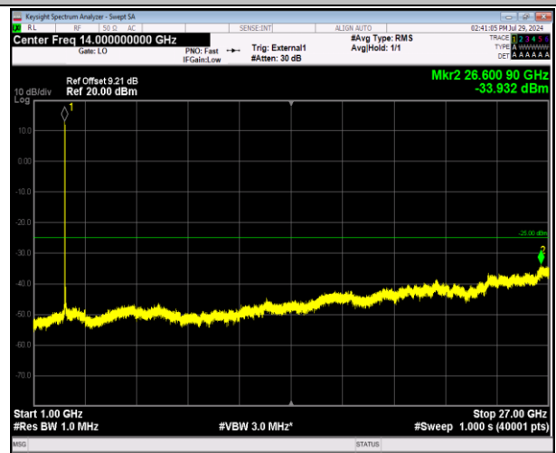
41-41-5MHz-20MHz-64QAM-64QAM-40528-40645-25RB#0 -100RB#0-1000~27000MHz-PASS
