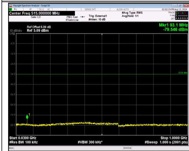
41-41-20MHz-5MHz-QPSK-QPSK-39750-39867-1RB#99-0RB#0-30~1000MHz-PASS
