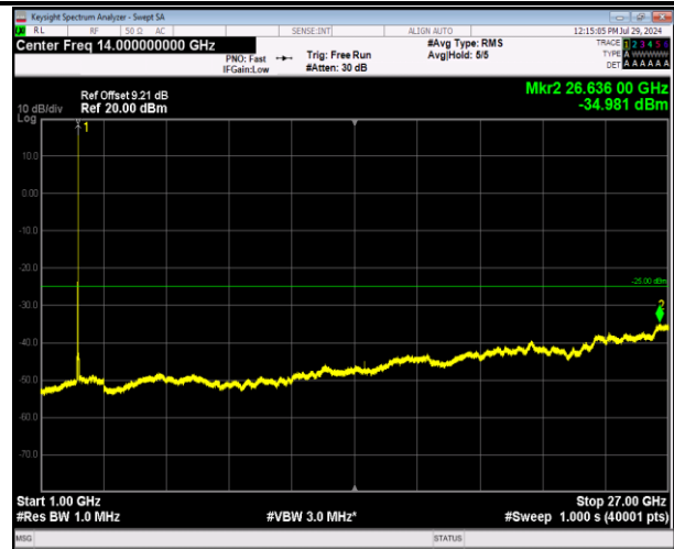
7-7-20MHz-20MHz-64QAM-64QAM-21152-21350-1RB#99- 0RB#0-1000~27000MHz-PASS
