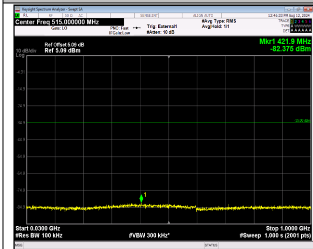
41-41-5MHz-20MHz-QPSK-QPSK-40528-40645-25RB#0-100RB#0-30~1000MHz-PASS
