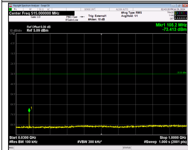
41-41-5MHz-20MHz-64QAM-64QAM-41373-41490-1RB# 0-1RB#99-30~1000MHz-PASS
