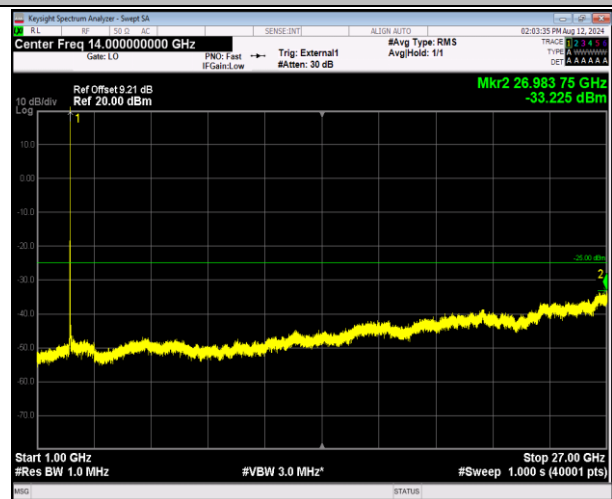
41-41-20MHz-5MHz-16QAM-16QAM-39750-39867-1RB#99 -ORB#0-1000~27000MHz-PASS
