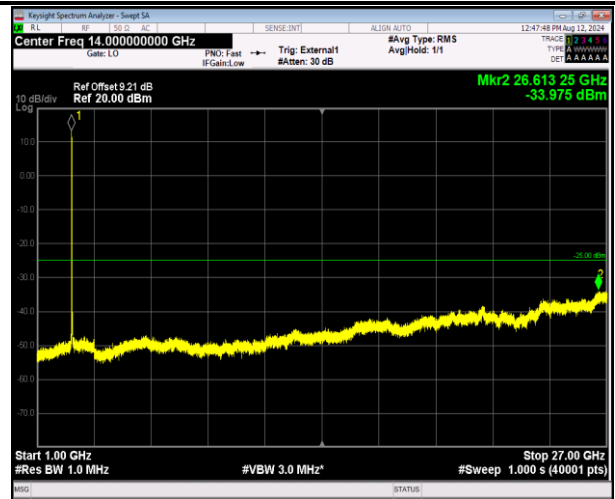
41-41-5MHz-20MHz-16QAM-16QAM-40528-40645-25RB#0-100RB#0-1000~27000MHz-PASS
