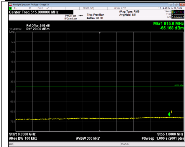
7-7-20MHz-20MHz-64QAM-64QAM-21152-21350-1RB#9 9-0RB#0-30~1000MHz-PASS
