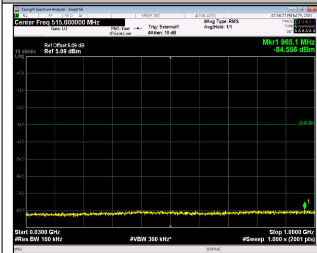
41-41-5MHz-20MHz-64QAM-64QAM-39683-39800-1RB# 0-1RB#99-30~1000MHz-PASS
