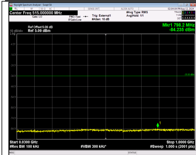
41-41-20MHz-5MHz-QPSK-QPSK-39750-39867-1RB#0-1RB#24-30~1000MHz-PASS
