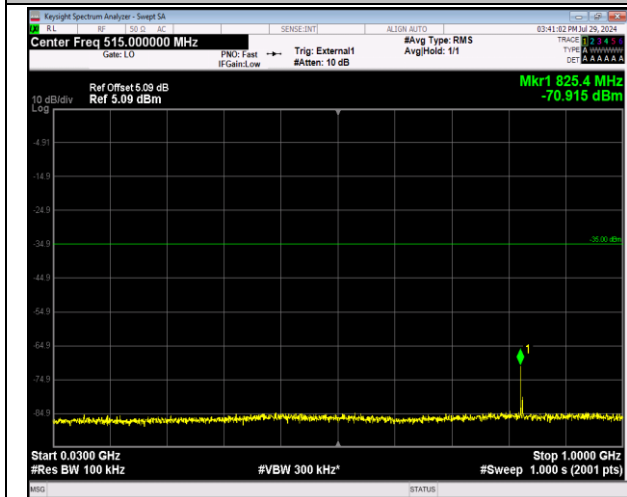
41-41-20MHz-5MHz-64QAM-64QAM-39750-39867-1RB# 0-1RB#24-30~1000MHz-PASS
