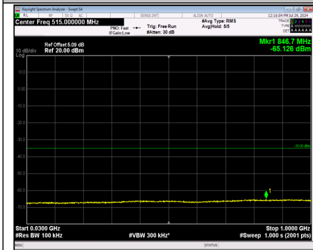
7-7-20MHz-20MHz-64QAM-64QAM-21152-21350-100RB #0-100RB#0-30~1000MHz-PASS
