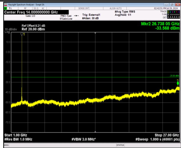
41-41-5MHz-20MHz-64QAM-64QAM-41373-41490-1RB#24 -ORB#0-1000~27000MHz-PASS
