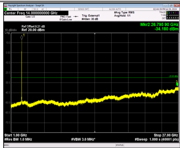
41-41-5MHz-20MHz-64QAM-64QAM-41373-41490-25RB#0 -100RB#0-1000~27000MHz-PASS
