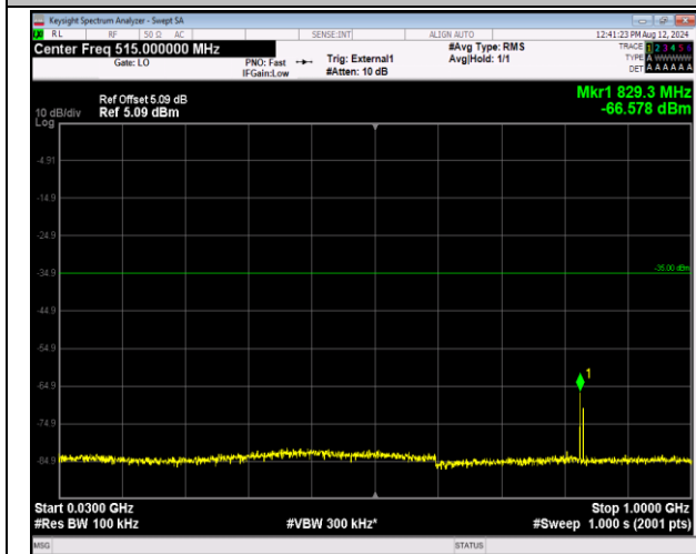
41-41-5MHz-20MHz-QPSK-QPSK-40528-40645-1RB#0-ORB#0-30~1000MHz-PASS
