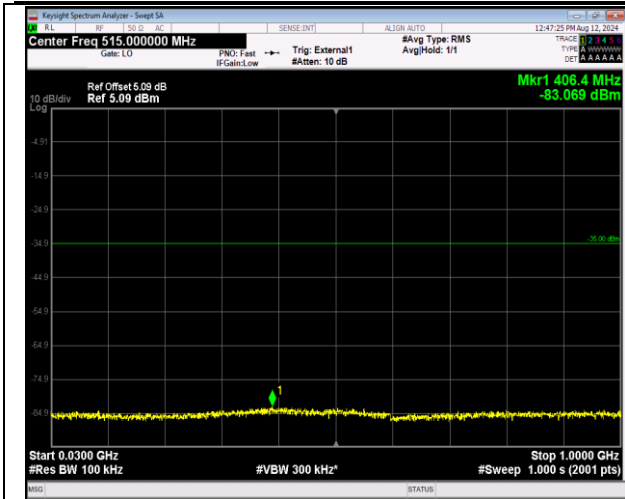
41-41-5MHz-20MHz-16QAM-16QAM-40528-40645-25RB#0-100RB#0-30~1000MHz-PASS
