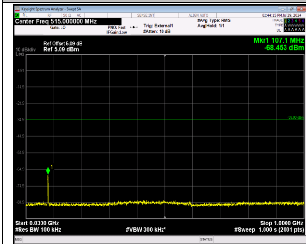
41-41-5MHz-20MHz-64QAM-64QAM-41373-41490-25RB #0-100RB#0-30~1000MHz-PASS
