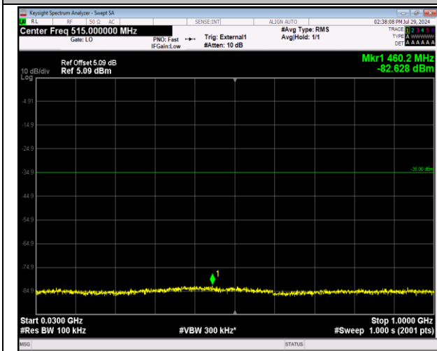
41-41-5MHz-20MHz-64QAM-64QAM-40528-40645-1RB#0-0RB#0-30~1000MHz-PASS
