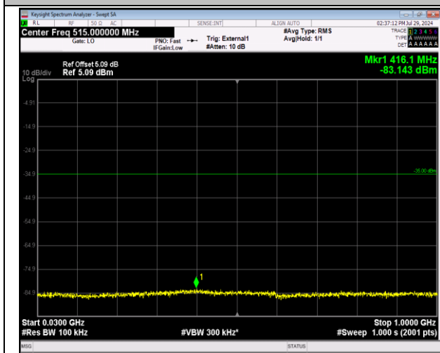
41-41-5MHz-20MHz-64QAM-64QAM-39683-39800-25RB #0-100RB#0-30~1000MHz-PASS
