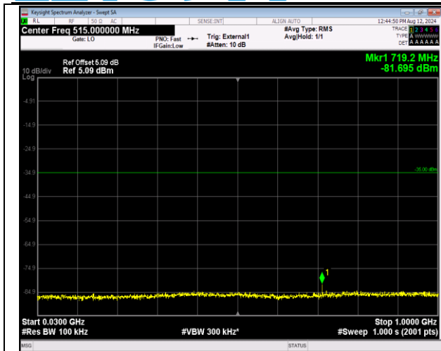
41-41-5MHz-20MHz-QPSK-QPSK-40528-40645-1RB#0-1RB#99-30~1000MHz-PASS
