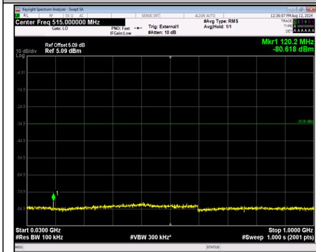
41-41-5MHz-20MHz-QPSK-QPSK-39683-39800-1RB#24-0RB#0-30~1000MHz-PASS
