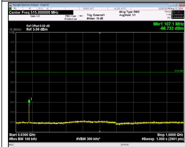
41-41-5MHz-20MHz-QPSK-QPSK-41373-41490-25RB#0-100RB#0-30~1000MHz-PASS
