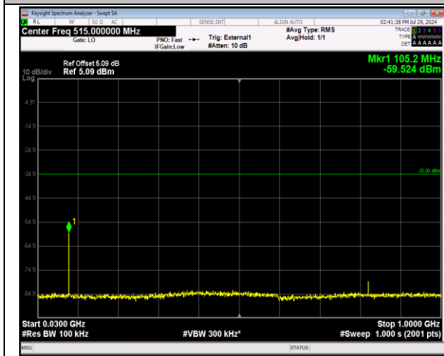
41-41-5MHz-20MHz-64QAM-64QAM-41373-41490-1RB# 0-0RB#0-30~1000MHz-PASS
