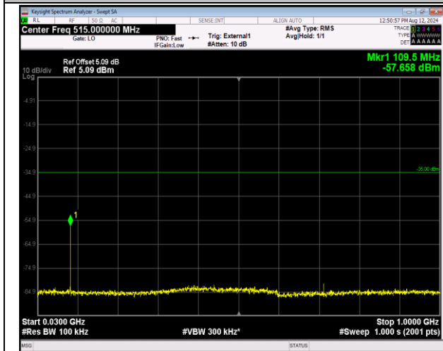
41-41-5MHz-20MHz-16QAM-16QAM-41373-41490-1RB# 24-ORB#0-30~1000MHz-PASS
