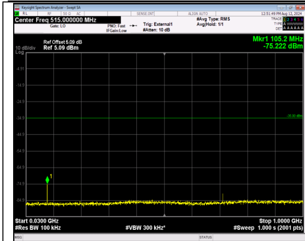
41-41-5MHz-20MHz-QPSK-QPSK-41373-41490-1RB#0-1RB#99-30~1000MHz-PASS
