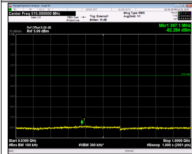
41-41-5MHz-20MHz-64QAM-64QAM-39683-39800-1RB# 0-0RB#0-30~1000MHz-PASS
