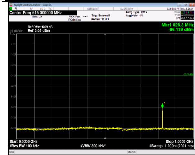
41-41-20MHz-5MHz-16QAM-16QAM-39750-39867-100R B#0-25RB#0-30~1000MHz-PASS
