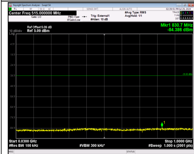
41-41-5MHz-20MHz-64QAM-64QAM-40528-40645-1RB#0-1RB#99-30~1000MHz-PASS
