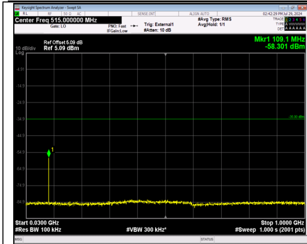
41-41-5MHz-20MHz-64QAM-64QAM-41373-41490-1RB# 24-ORB#0-30~1000MHz-PASS
