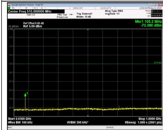
41-41-5MHz-20MHz-16QAM-16QAM-41373-41490-1RB# 0-1RB#99-30~1000MHz-PASS
