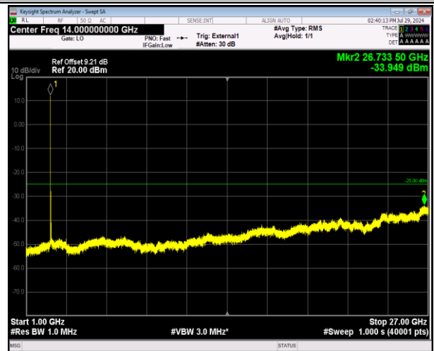
41-41-5MHz-20MHz-64QAM-64QAM-40528-40645-1RB#0-1RB#99-1000~27000MHz-PASS
