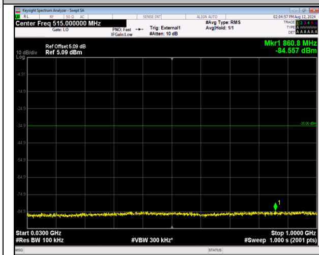
41-41-20MHz-5MHz-16QAM-16QAM-39750-39867-1RB# 0-1RB#24-30~1000MHz-PASS
