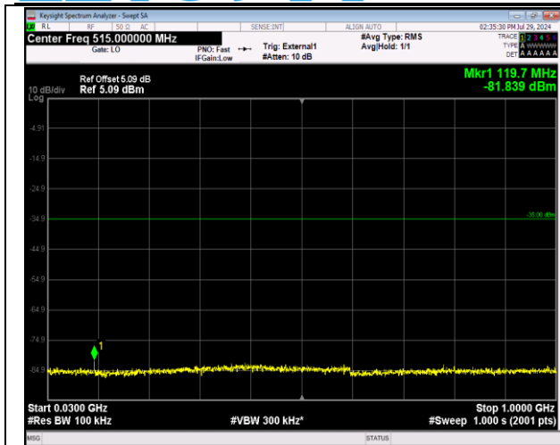
41-41-5MHz-20MHz-64QAM-64QAM-39683-39800-1RB# 24-ORB#0-30~1000MHz-PASS
