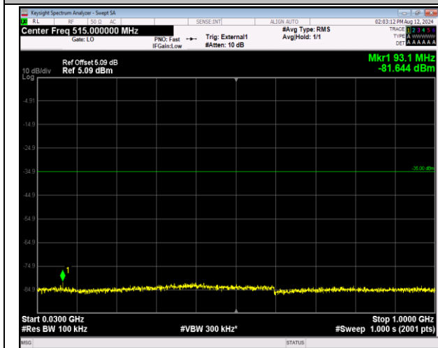
41-41-20MHz-5MHz-16QAM-16QAM-39750-39867-1RB# 99-ORB#0-30~1000MHz-PASS
