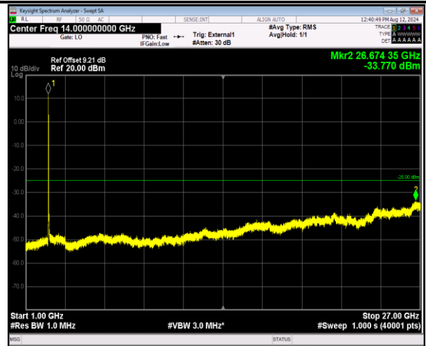
41-41-5MHz-20MHz-16QAM-16QAM-39683-39800-25RB#0 -100RB#0-1000~27000MHz-PASS
