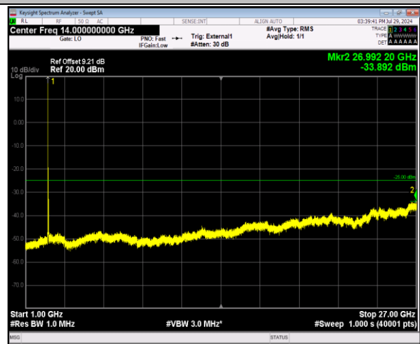
41-41-20MHz-5MHz-64QAM-64QAM-39750-39867-1RB#0- 0RB#0-1000~27000MHz-PASS
