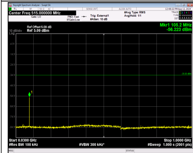
41-41-5MHz-20MHz-QPSK-QPSK-41373-41490-1RB#0-ORB#0-30~1000MHz-PASS
