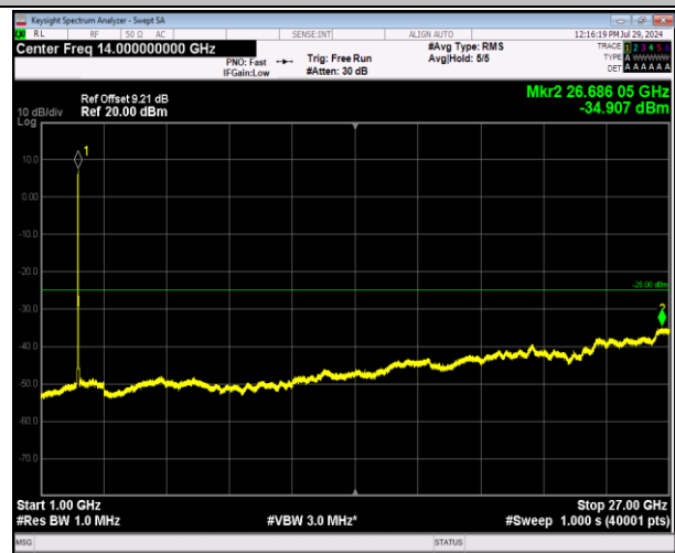
7-7-20MHz-20MHz-64QAM-64QAM-21152-21350-100RB#0 -100RB#0-1000~27000MHz-PASS
