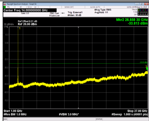
41-41-5MHz-20MHz-16QAM-16QAM-41373-41490-1RB#24 -ORB#0-1000~27000MHz-PASS
