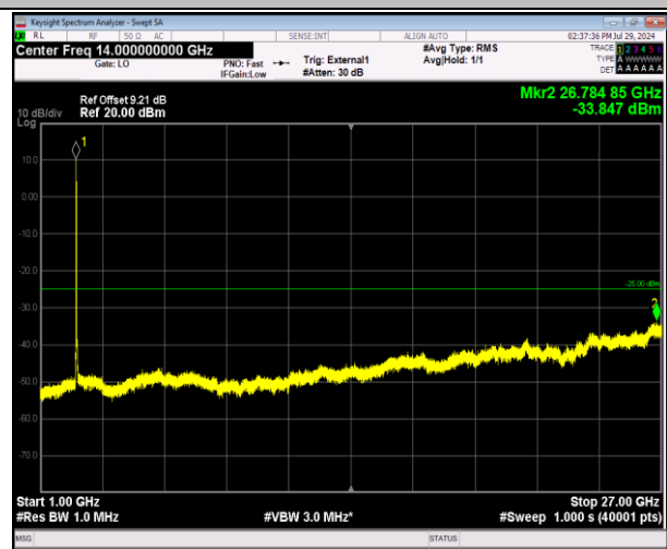
41-41-5MHz-20MHz-64QAM-64QAM-39683-39800-25RB#0 -100RB#0-1000~27000MHz-PASS
