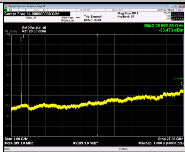
41-41-20MHz-5MHz-16QAM-16QAM-39750-39867-1RB#0- 1RB#24-1000~27000MHz-PASS
