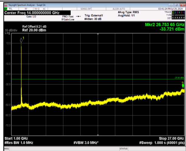
41-41-20MHz-5MHz-64QAM-64QAM-39750-39867-1RB#0- 1RB#24-1000~27000MHz-PASS
