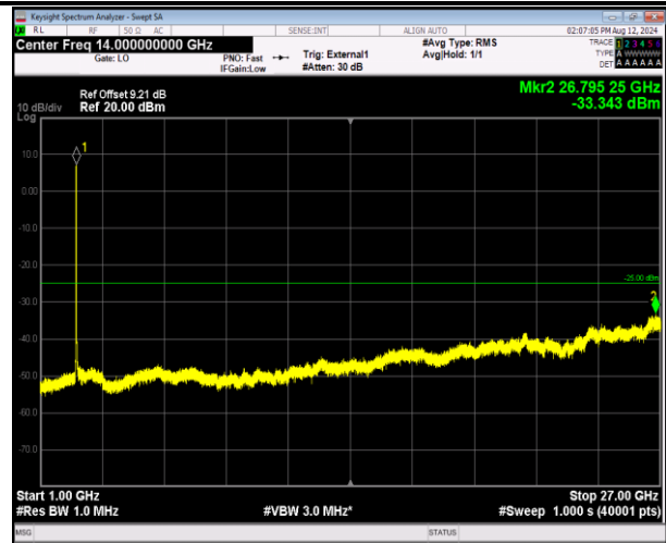
41-41-20MHz-5MHz-16QAM-16QAM-39750-39867-100RB# 0-25RB#0-1000~27000MHz-PASS
