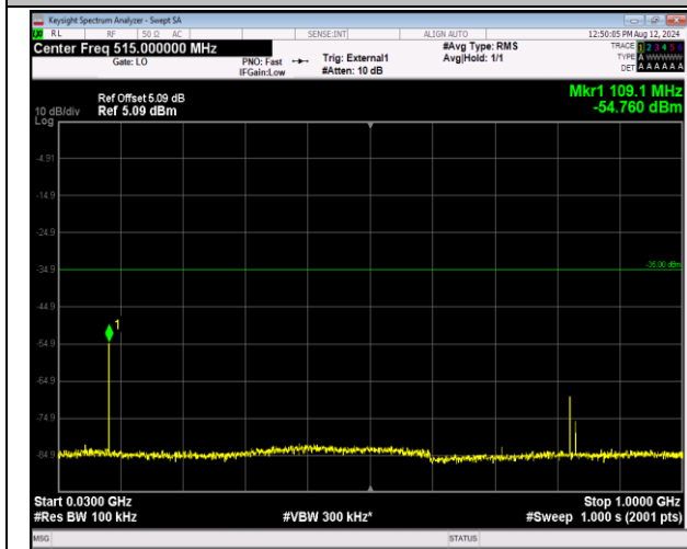
41-41-5MHz-20MHz-QPSK-QPSK-41373-41490-1RB#24-0-0RB#0-30~1000MHz-PASS
