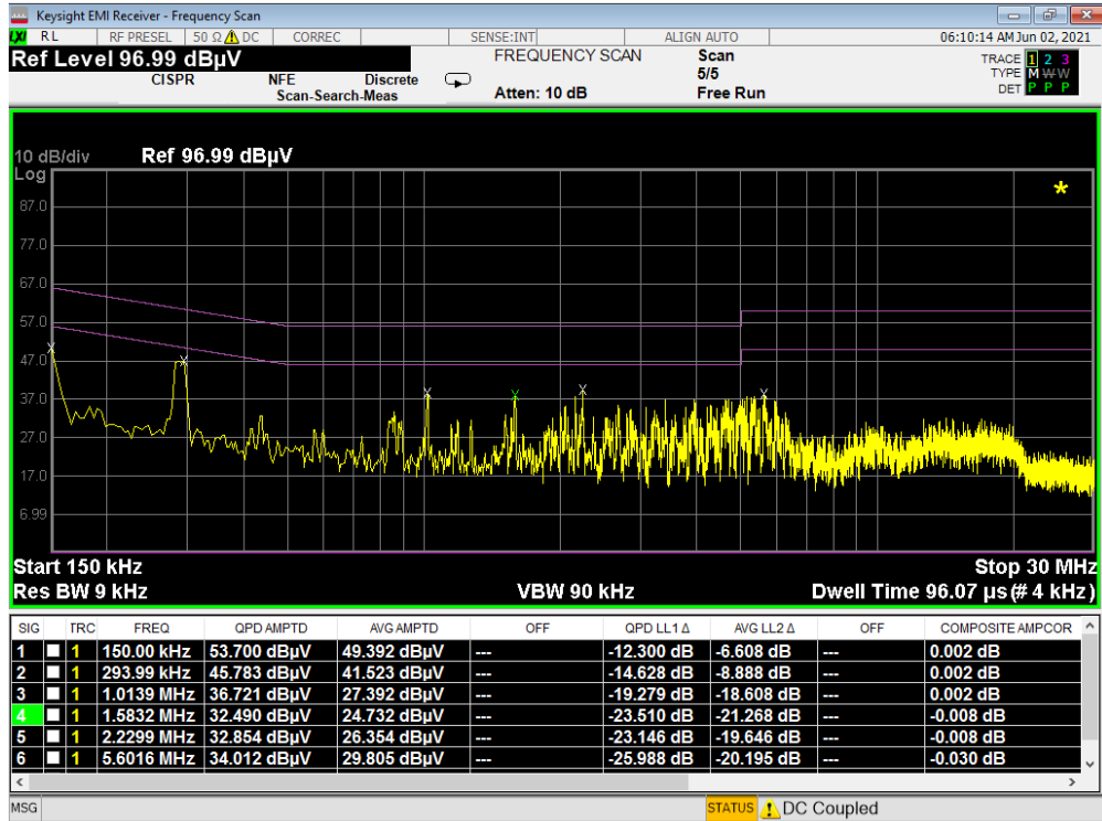
Plot 7-14. Line-Conducted Test Plot (L1) – Digitizer – Click
