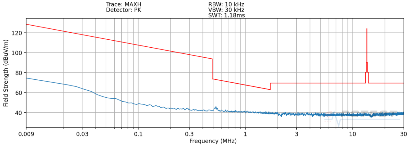
Plot 7-7. Radiated Spurious Plot 9kHz – 30MHz (Pol. X – Digitizer – Click)
