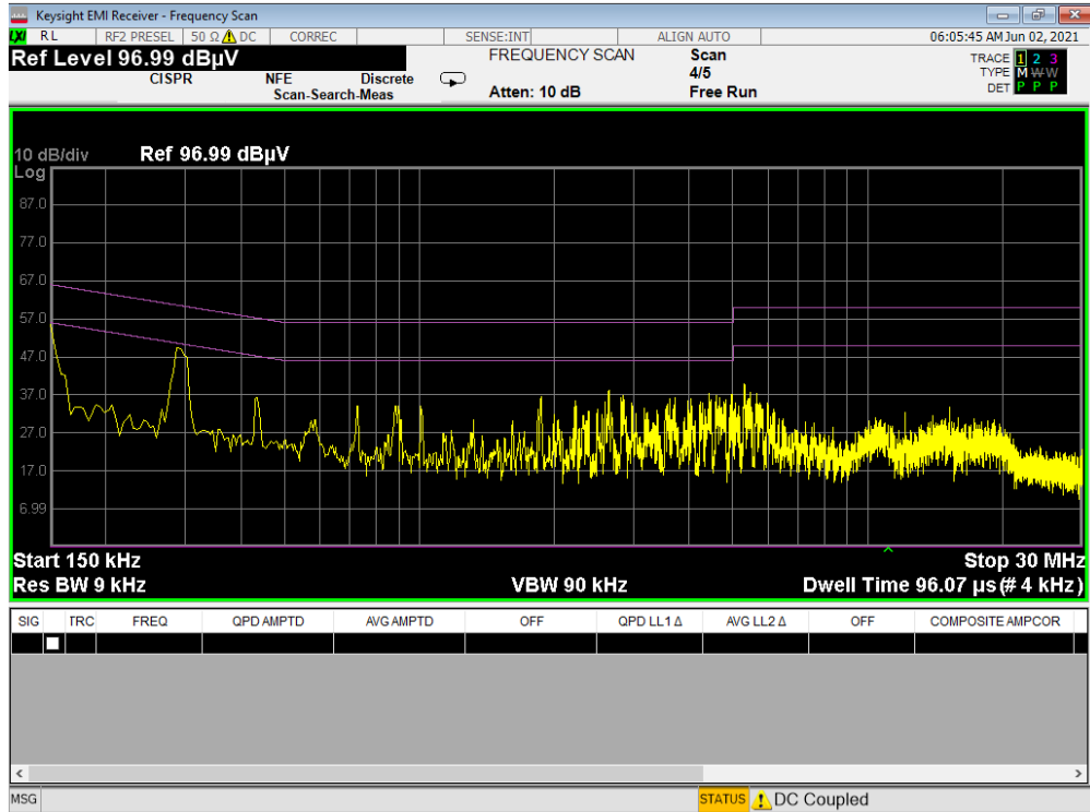
Plot 7-12. Line-Conducted Test Plot (L1) – Digitizer – Hover
