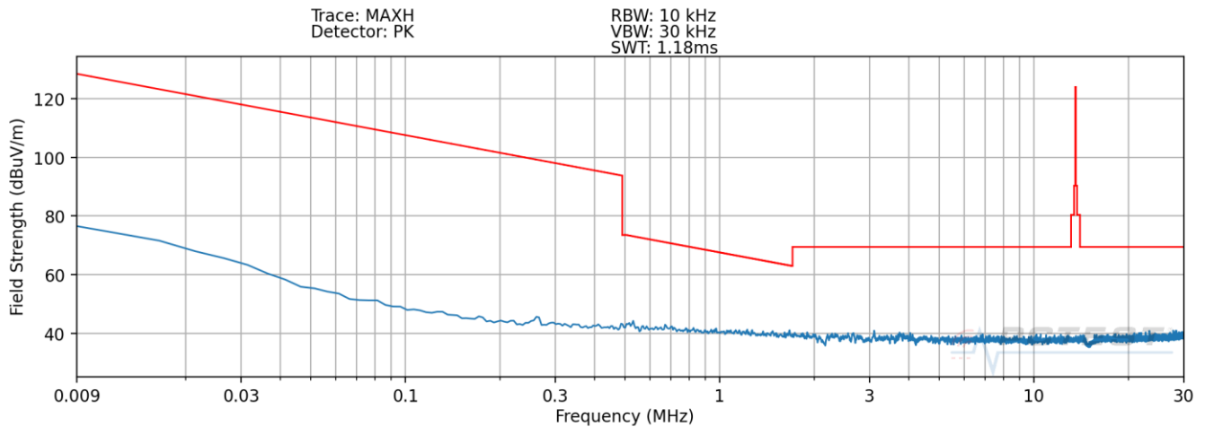
Plot 7-9. Radiated Spurious Plot 9kHz – 30MHz (Pol. Z – Digitizer – Click)
