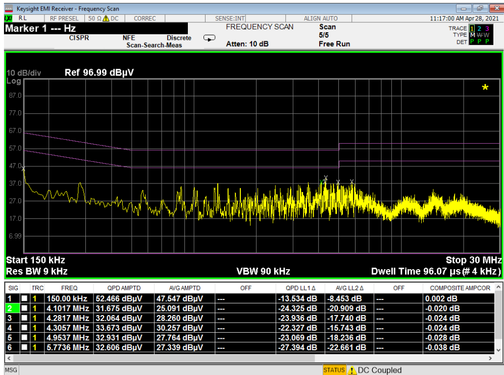
Plot 7-11. Line-Conducted Test Plot (N) - Device to Device WPT
