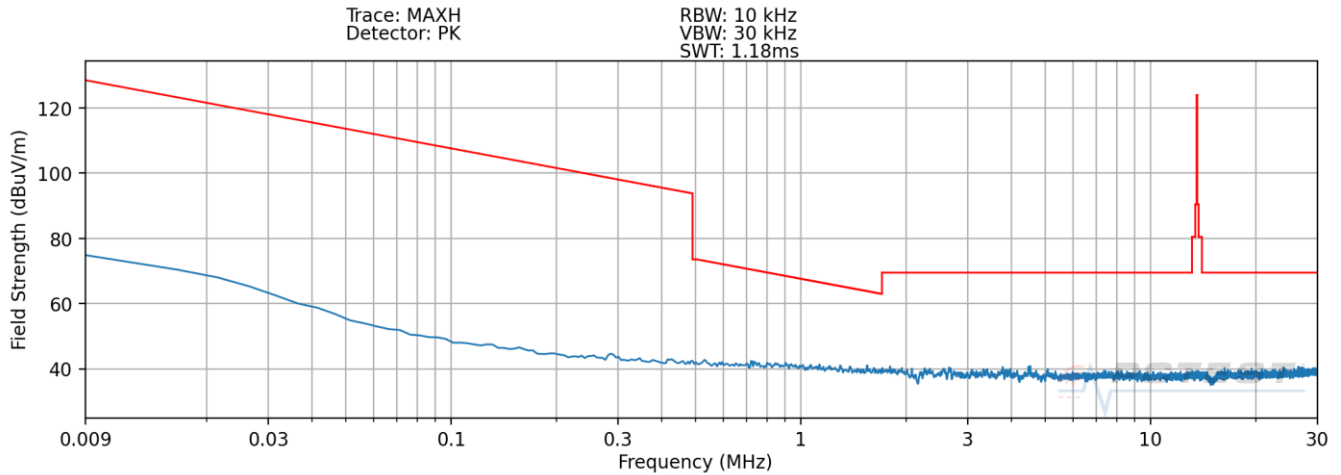
Plot 7-8 Radiated Spurious Plot 9kHz – 30MHz (Pol. Y – Digitizer – Click)
