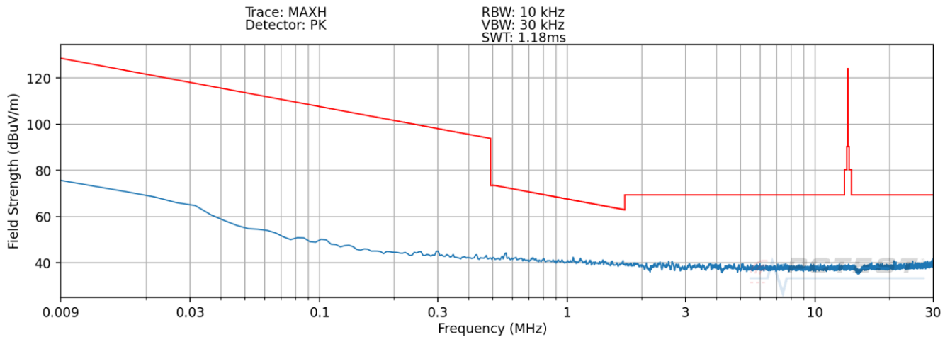
Plot 7-6. Radiated Spurious Plot 9kHz – 30MHz (Pol. Z – Digitizer – Hover)
