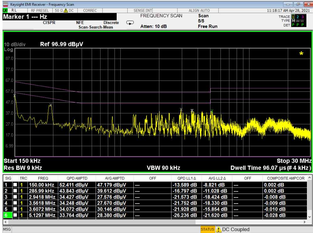
Plot 7-10. Line-Conducted Test Plot (L1) - Device to Device WPT
