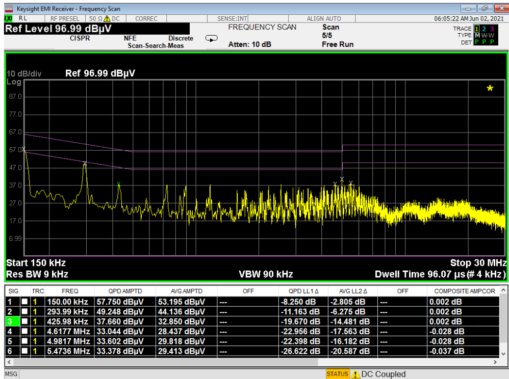
Plot 7-13. Line-Conducted Test Plot (N) – Digitizer – Hover
