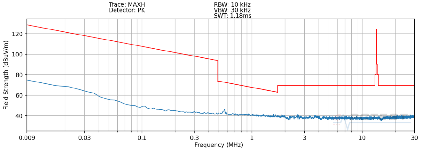
Plot 7-4. Radiated Spurious Plot 9kHz – 30MHz (Pol. X – Digitizer – Hover)
