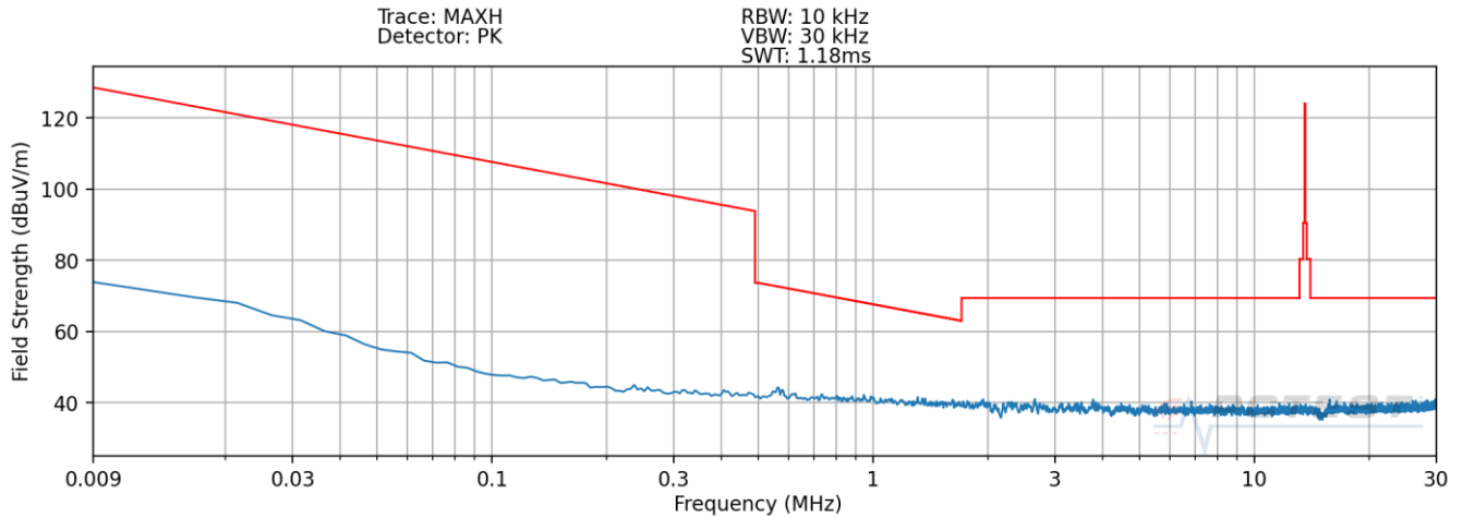
Plot 7-5 Radiated Spurious Plot 9kHz – 30MHz (Pol. Y – Digitizer – Hover)
