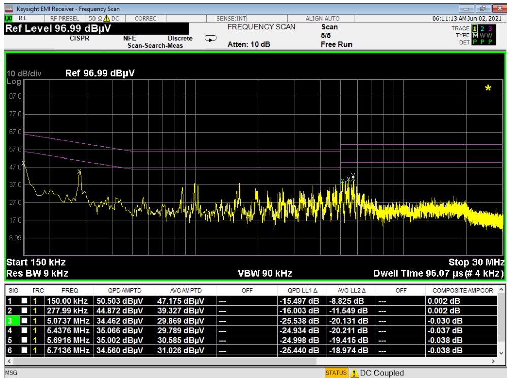
Plot 7-15. Line-Conducted Test Plot (N) – Digitizer – Click
