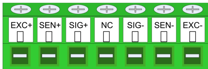
Figure 2-9: Load Cell Termination
