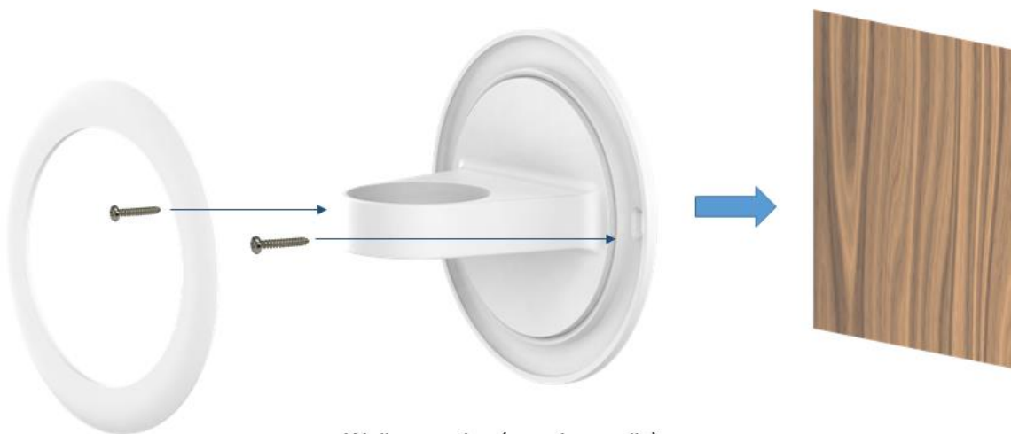
Wall mounting (wooden walls)
