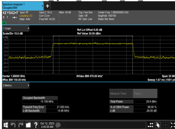
N2(15M)_CP-OFDM_QPSK Outer Full Mid CH
