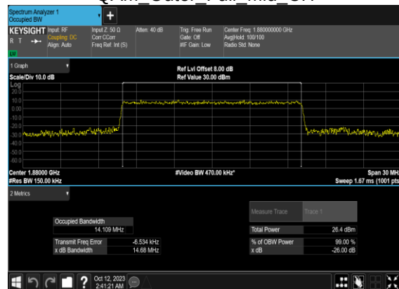
N2(15M)_CP-OFDM_256 QAM Outer Full Mid CH
