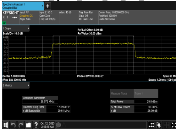
N2(30M)_CP-OFDM_QPSK Outer Full Mid CH
