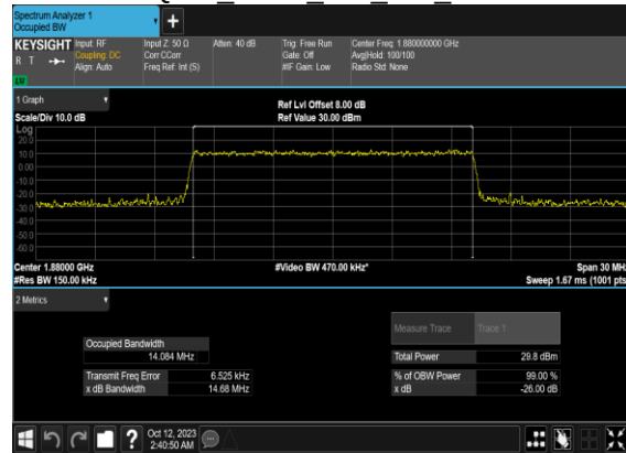
N2(15M)_CP-OFDM_16 QAM Outer Full Mid CH
