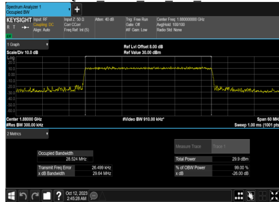
N2(30M)_CP-OFDM_16 QAM Outer Full Mid CH
