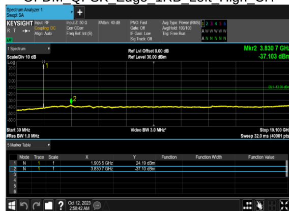
N2(5M)_DFT-s- OFDM QPSK Edge 1RB Left High CH
