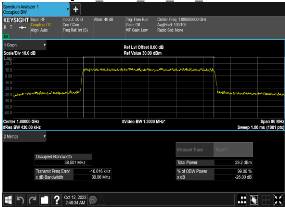
N2(40M)_CP-OFDM_64 QAM_Outer_Full_Mid_CH
