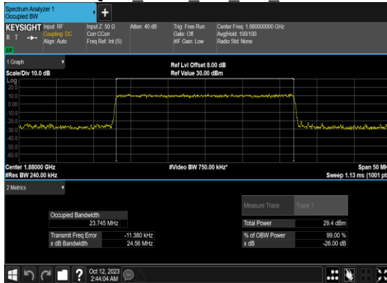
N2(25M)_CP-OFDM_64 QAM Outer Full Mid CH
