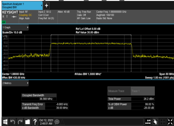
N2(40M)_CP-OFDM_256 QAM_Outer_Full_Mid_CH
