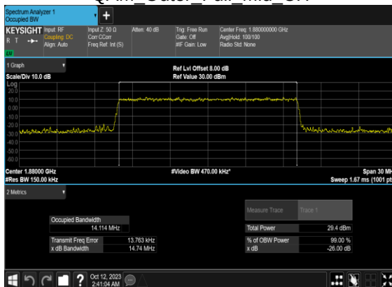
N2(15M)_CP-OFDM_64 QAM Outer Full Mid CH
