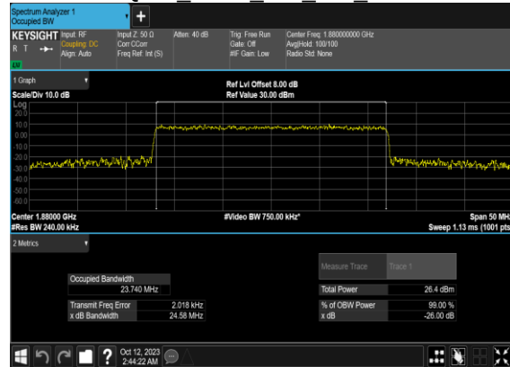
N2(25M)_CP-OFDM_256 QAM Outer Full Mid CH
