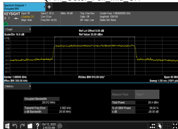
N2(30M)_CP-OFDM_256 QAM Outer Full Mid CH
