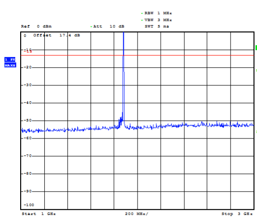
GSM 1900 CH-Low 1GHz~3GHz
