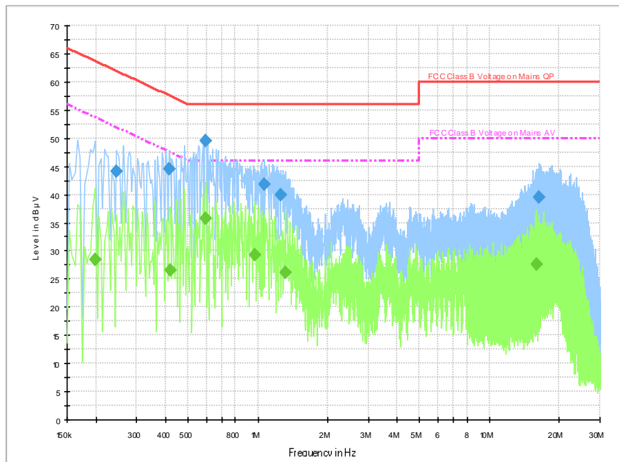
Fig.B.8.1 AC Powerline Conducted Emission-BLE
