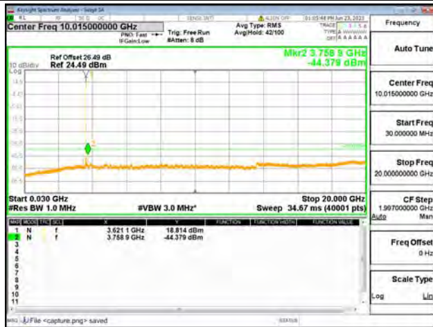
Band48-30M-20G / 10MHz / Mid CH / QPSK
