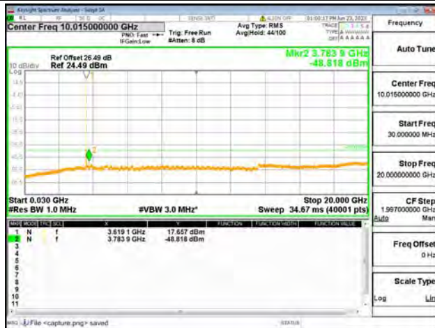
Band48-30M-20G / 15MHz / Mid CH / QPSK
