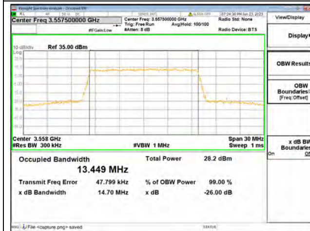
Band48 / 15MHz / 64QAM/ Low CH
