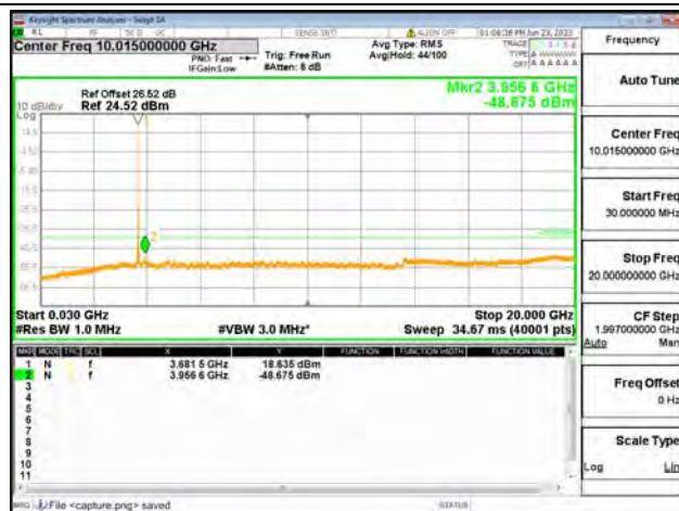
Band48-30M-20G / 20MHz / High CH / QPSK
