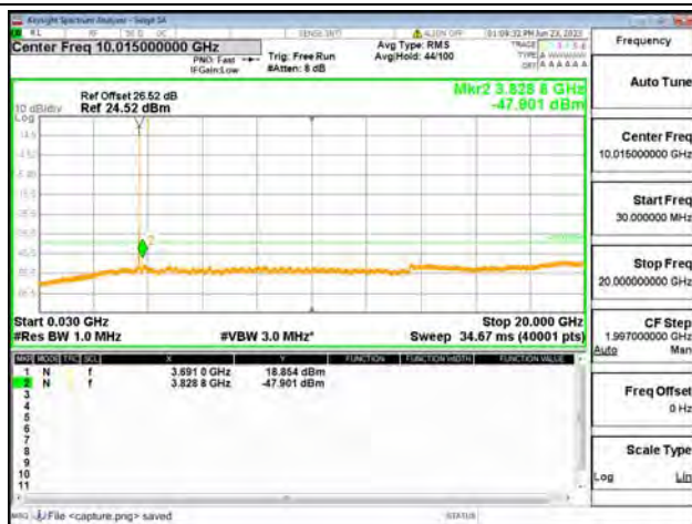
Band48-30M-20G / 10MHz / High CH / QPSK
