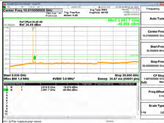
Band48-30M-20G / 20MHz / Mid CH / QPSK
