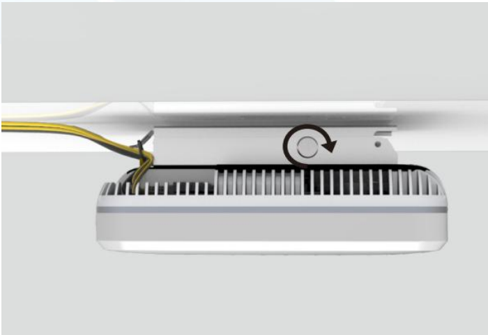
Figure 23. Tighten N2RU
