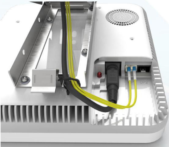
Figure 32. Wire Connection Diagram
