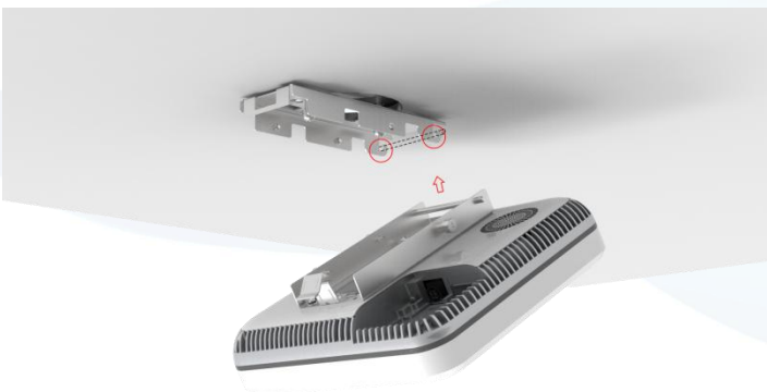
Figure 31. Buckle up
