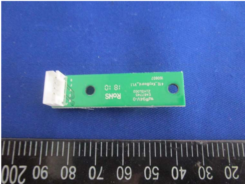
EUT – Switch Board Bottom View
