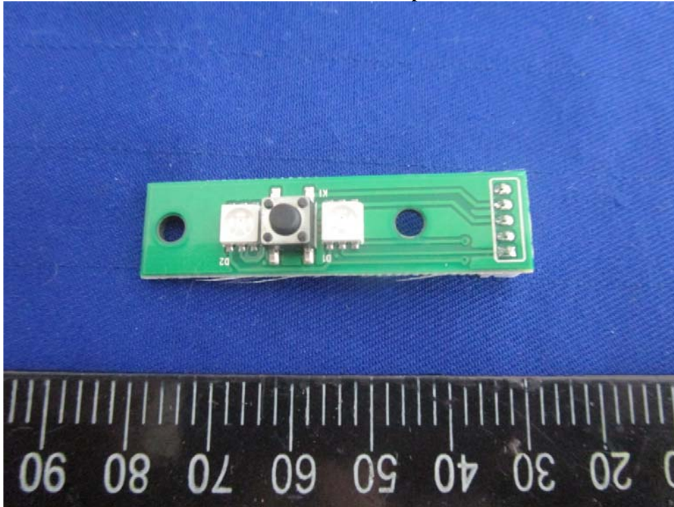
EUT – Switch Board Top View
