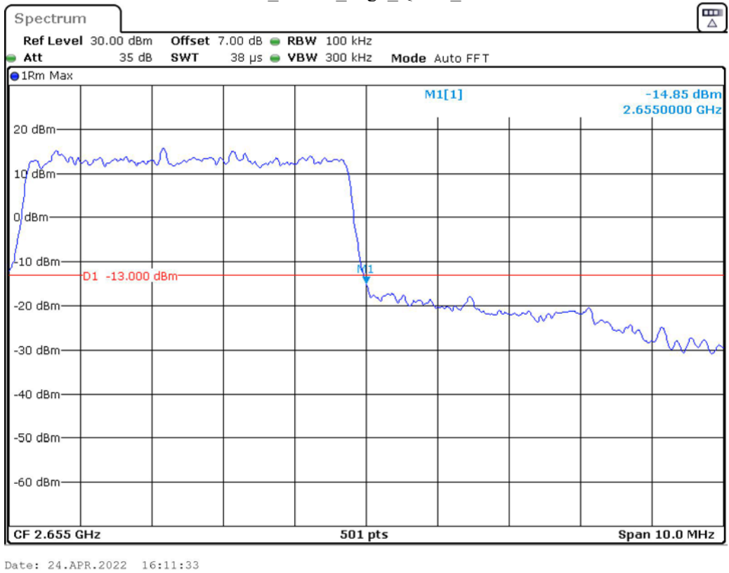
Band 41_5 MHz_High_QPSK_RB25#0
