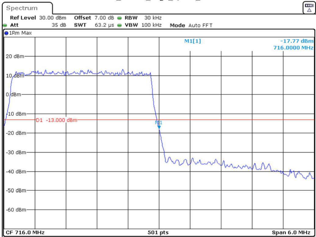
Band 12_3 MHz_High_QPSK_RB15#0
