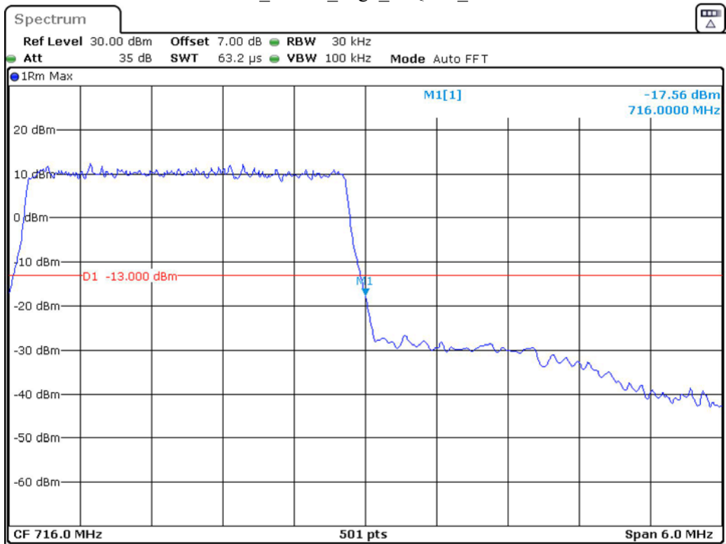
Band 12_3 MHz_High_16QAM_RB15#0
