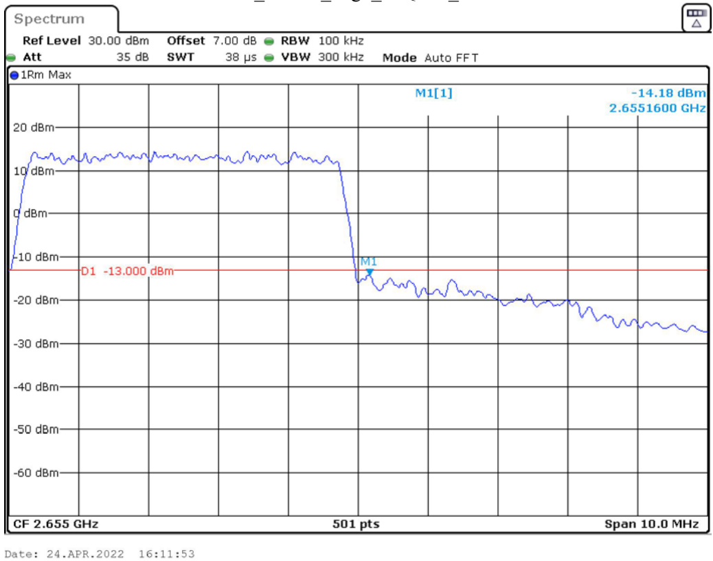
Band 41_5 MHz_High_16QAM_RB25#0
