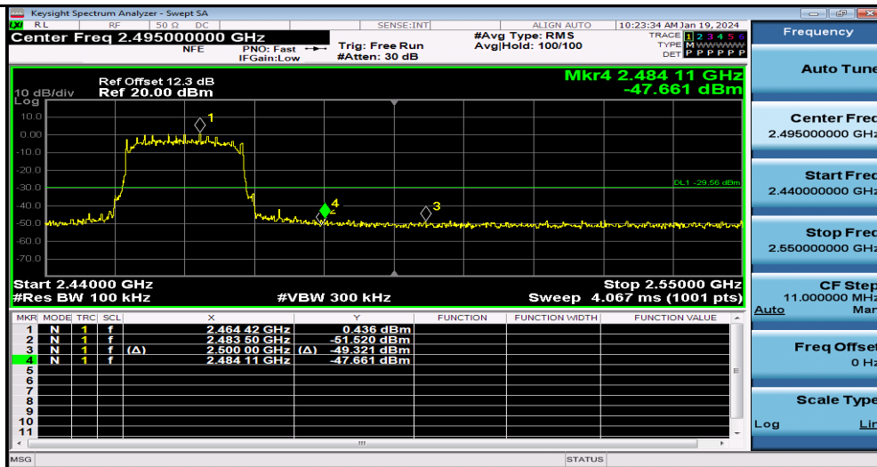
11N20SISO_Ant1_High_2462
