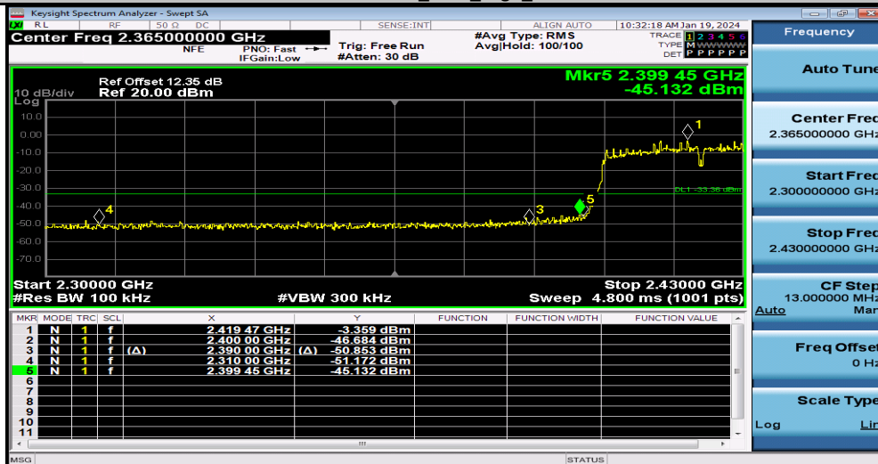
11N40SISO_Ant1_Low_2422
