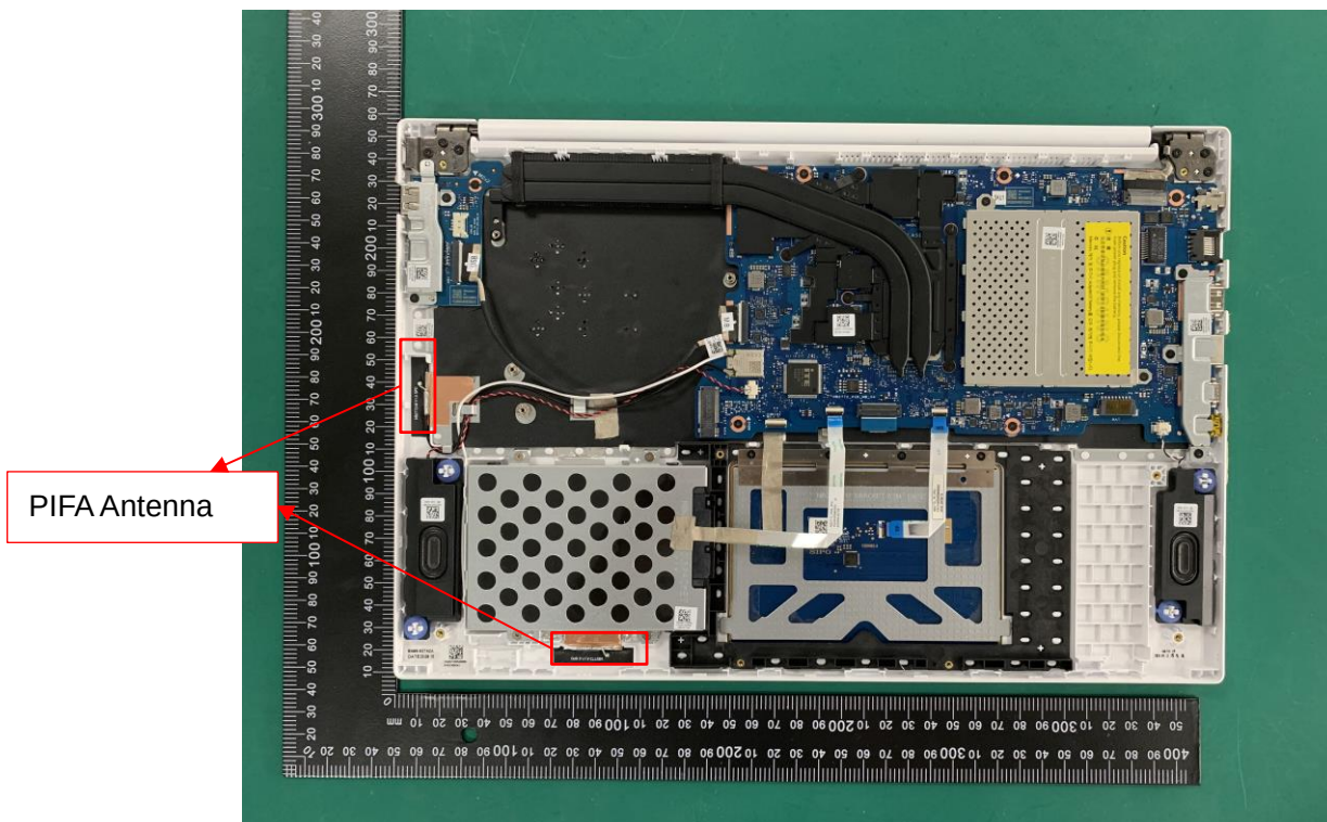
EUT UNCOVER VIEW (With GPU Version)
