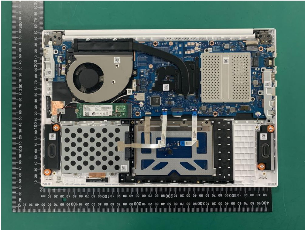
EUT UNCOVER VIEW (Without GPU Version)
