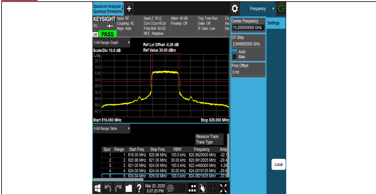
Band26(814-824)-3MHz-QPSK-26775-1RB#14-PASS
