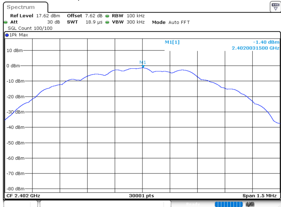
Tx. Spurious NVNT GFSK 2402MHz Ant1 Ref
