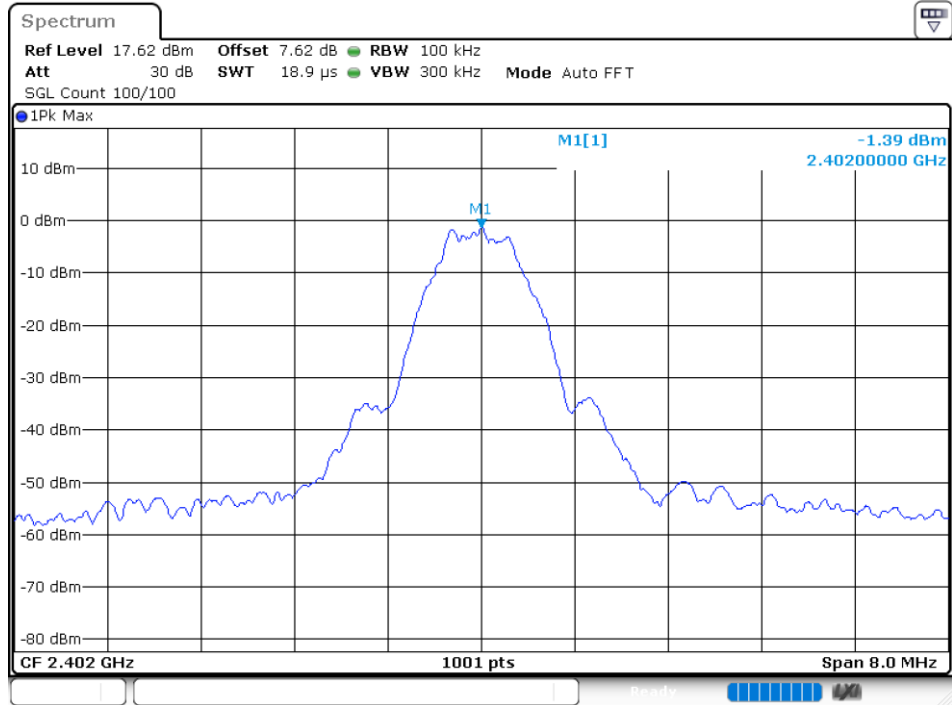
Band Edge NVNT GFSK 2402MHz Ant1 Emission
