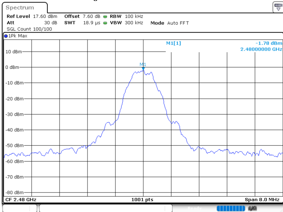
Band Edge NVNT GFSK 2480MHz Ant1 Emission
