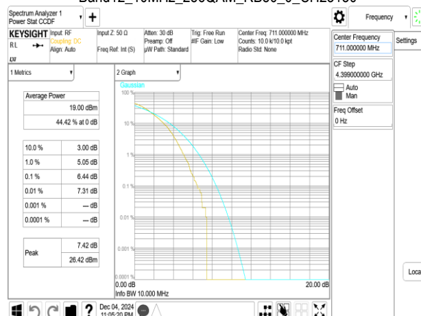
Band12_10MHz_256QAM_RB50_0_CH23130
