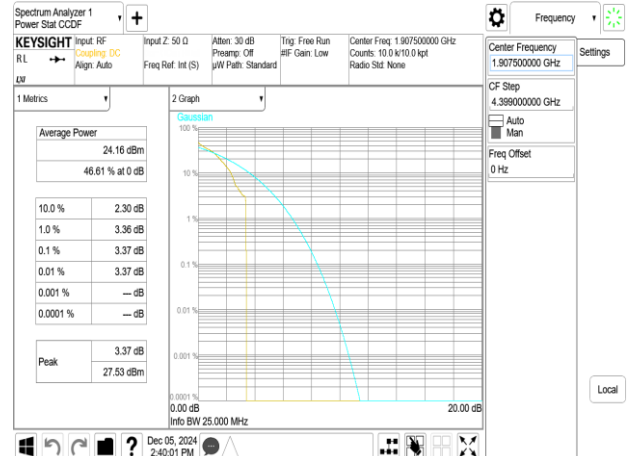
Band25_15MHz_QPSK_RB1_0_CH26615
