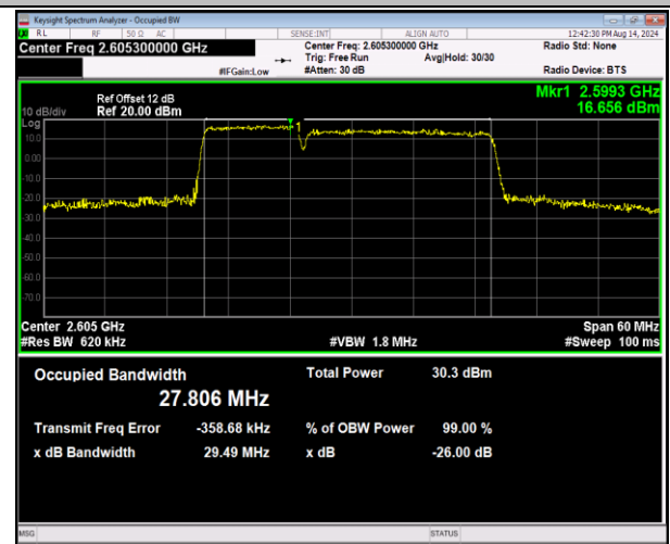
41-41-10MHz-20MHz-QPSK-QPSK-40646-40790-50RB#0-100RB#0-PASS
