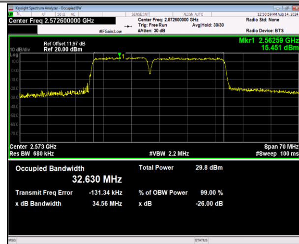
41-41-15MHz-20MHz-16QAM-16QAM-40318-40489-75RB#0-100RB#0-PASS
