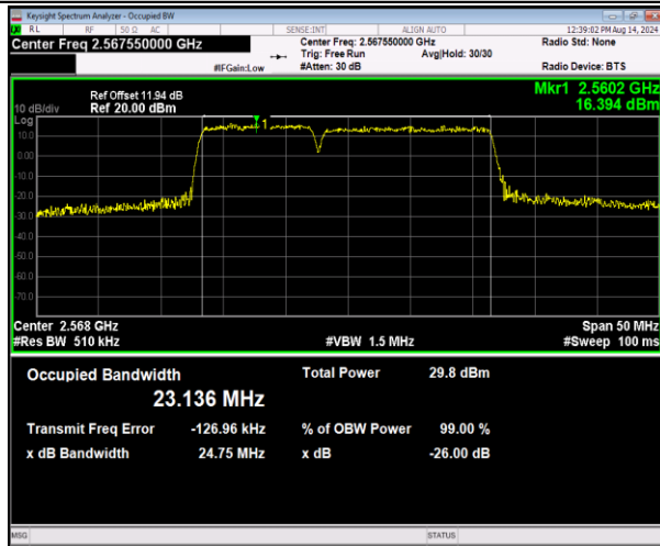
41-41-10MHz-15MHz-16QAM-16QAM-40293-40413-50RB#0-75RB#0-PASS
