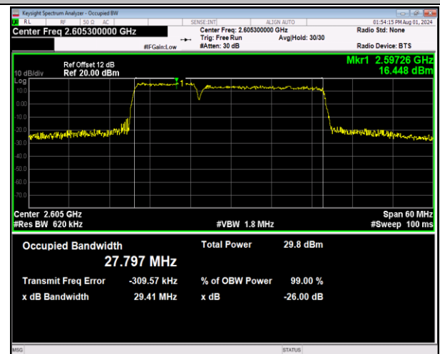
41-41-10MHz-20MHz-64QAM-64QAM-40646-40790-50RB#0-100RB#0-PASS
