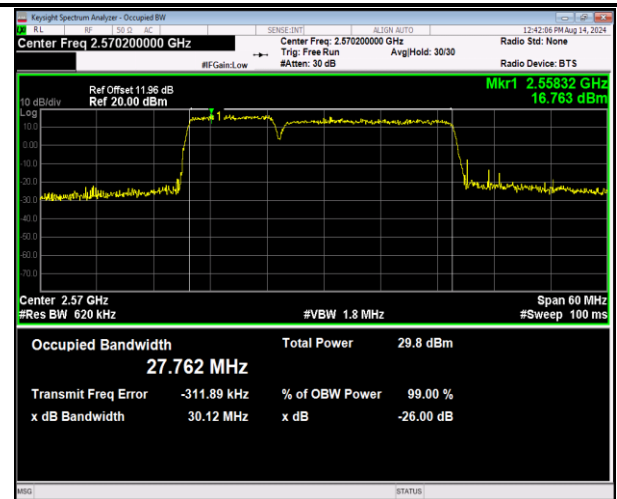
41-41-10MHz-20MHz-16QAM-16QAM-40295-40439-50RB#0-100RB#0-PASS
