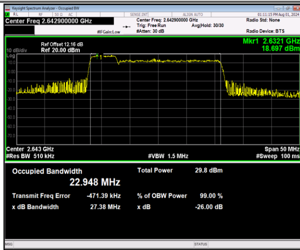
41-41-5MHz-20MHz-64QAM-64QAM-41023-41140-25RB#0-100RB#0-PASS
