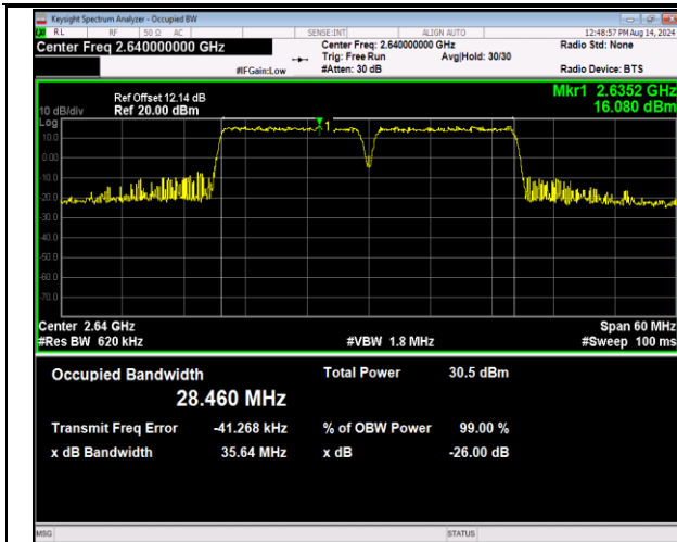
41-41-15MHz-15MHz-QPSK-QPSK-41015-41165-75RB#0-75RB#0-PASS
