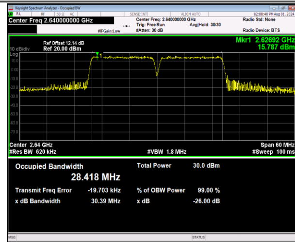
41-41-15MHz-15MHz-64QAM-64QAM-41015-41165-75RB#0-75RB#0-PASS
