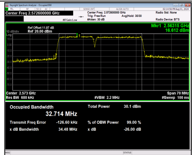
41-41-15MHz-20MHz-64QAM-64QAM-40318-40489-75RB#0-100RB#0-PASS
