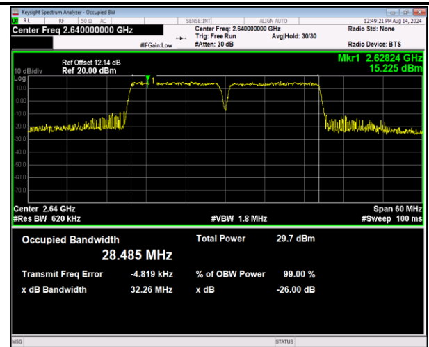
41-41-15MHz-15MHz-16QAM-16QAM-41015-41165-75RB#0-75RB#0-PASS
