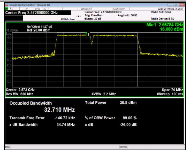
41-41-15MHz-20MHz-QPSK-QPSK-40318-40489-75RB#0-100RB#0-PASS
